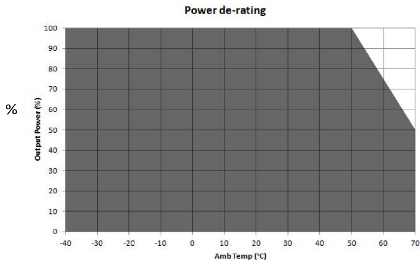
Figure 1. Derating Curve for all Outputs
