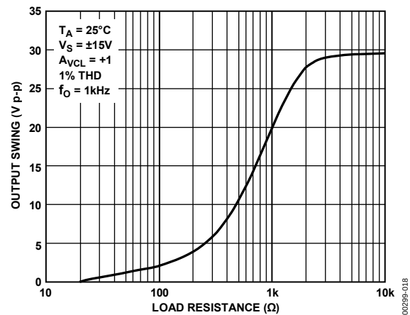
Figure 18. Maximum Output Swing vs. Load Resistance
