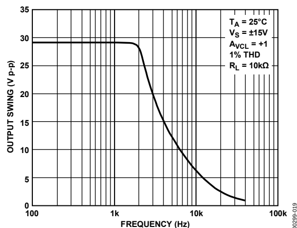
Figure 19. Maximum Output Swing vs. Frequency
