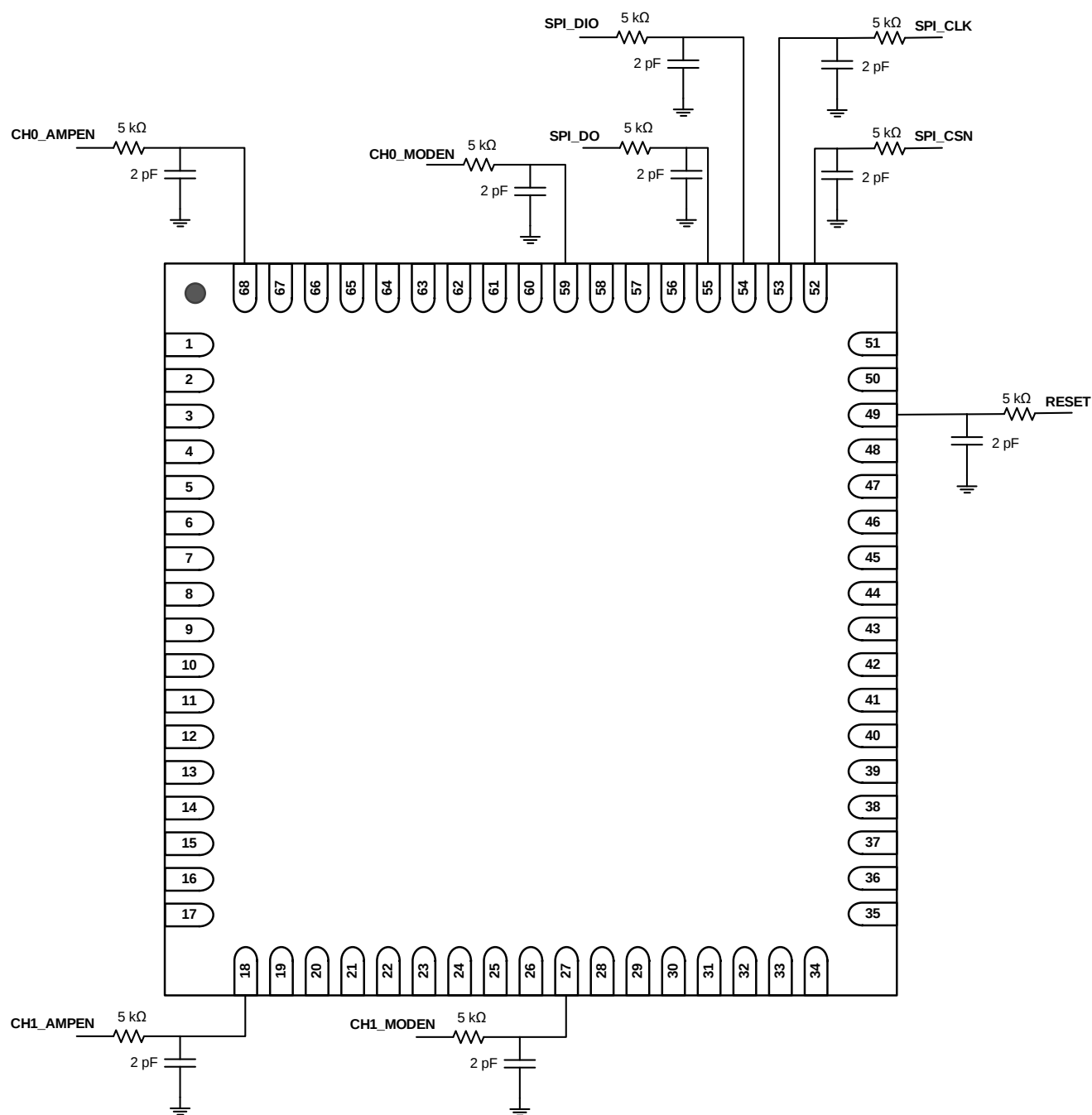
Figure 101. Control Pin Interface
