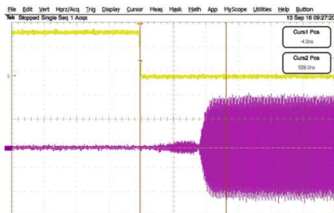
Figure 84. Switching Time OFF to ON
