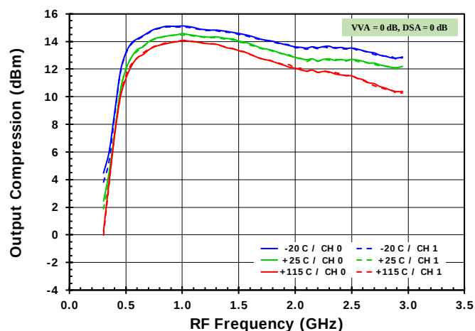
Figure 59. Output P1dB vs Frequency (+3.3V)
