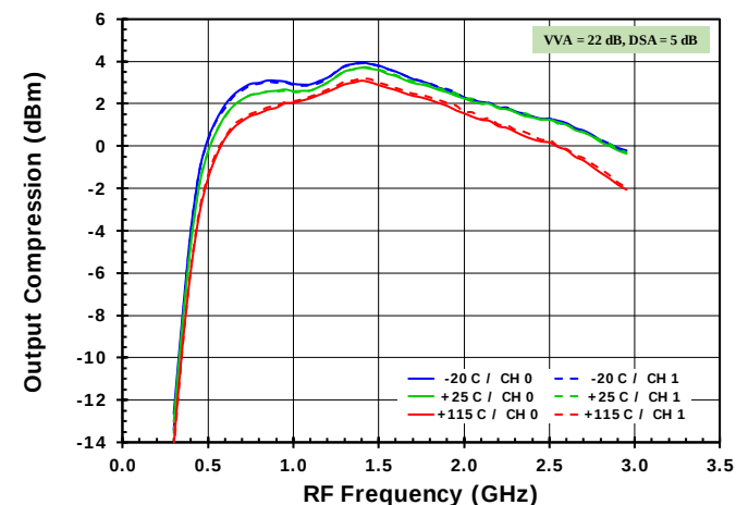
Figure 65. Output P1dB vs Frequency (+3.3V)
