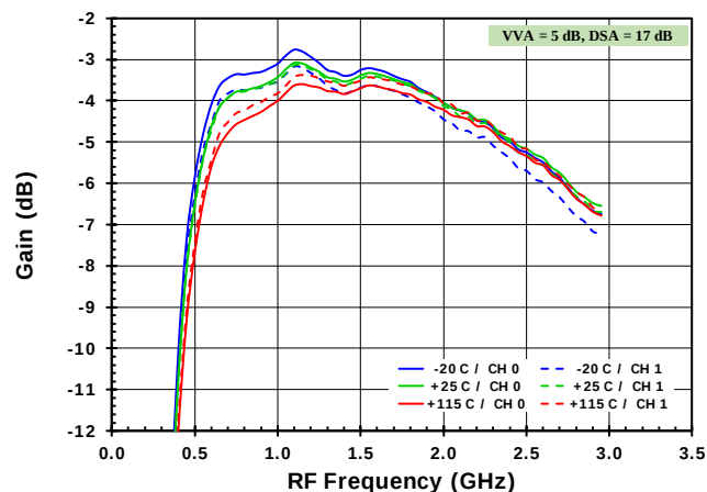
Figure 25. Gain versus Frequency (+3.3V)
