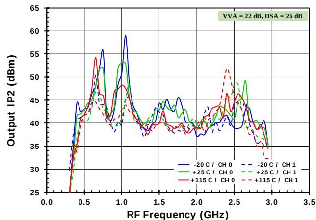
Figure 55. OIP2 versus Frequency (+3.3V)
