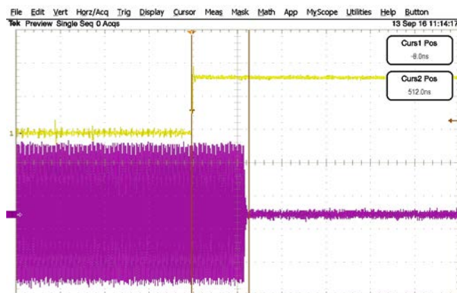
Figure 19. DSA Minimum to Maximum Switching (+3.3V, +25°C)
