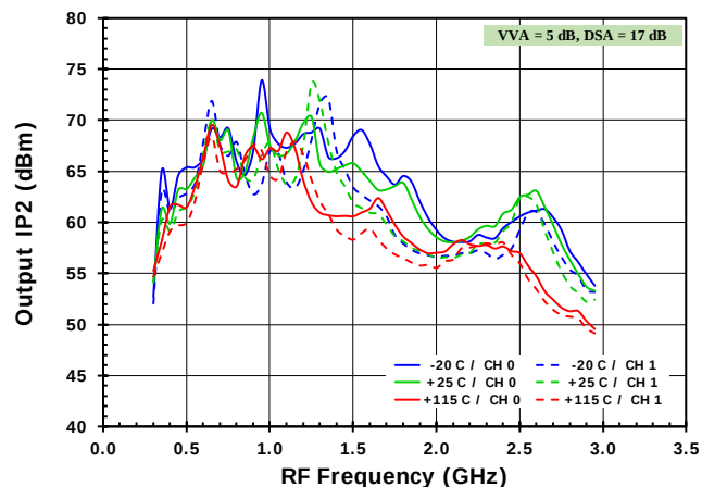
Figure 49. OIP2 versus Frequency (+3.3V)
