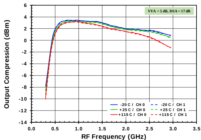
Figure 61. Output P1dB vs Frequency (+3.3V)
