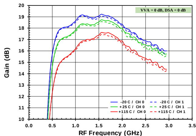
Figure 23. Gain versus Frequency (+3.3V)
