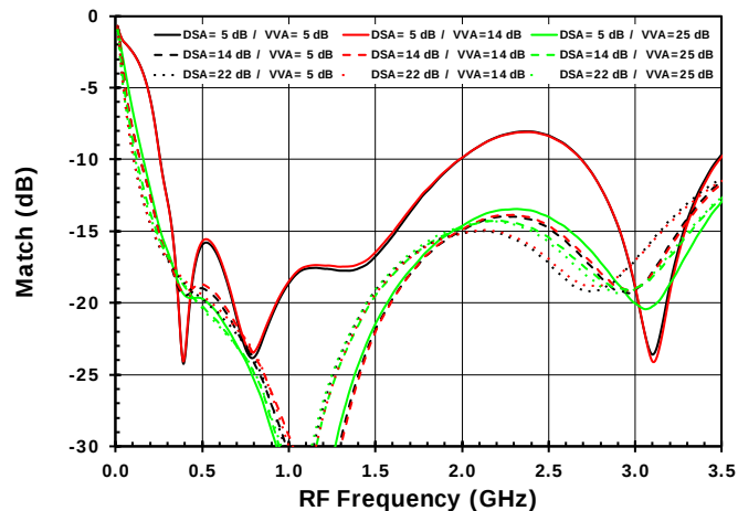
Figure 8. RF Output Return Loss (+25 °C)
