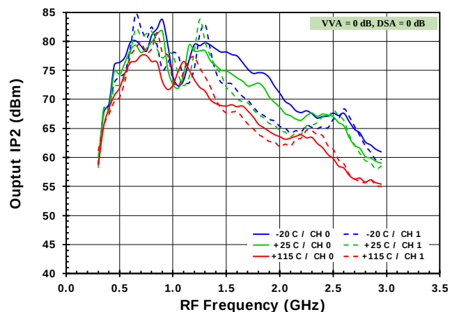
Figure 47. OIP2 versus Frequency (+3.3V)
