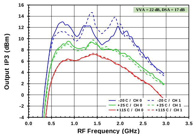
Figure 43. OIP3 versus Frequency (+3.3V)
