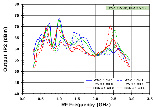
Figure 53. OIP2 versus Frequency (+3.3V)
