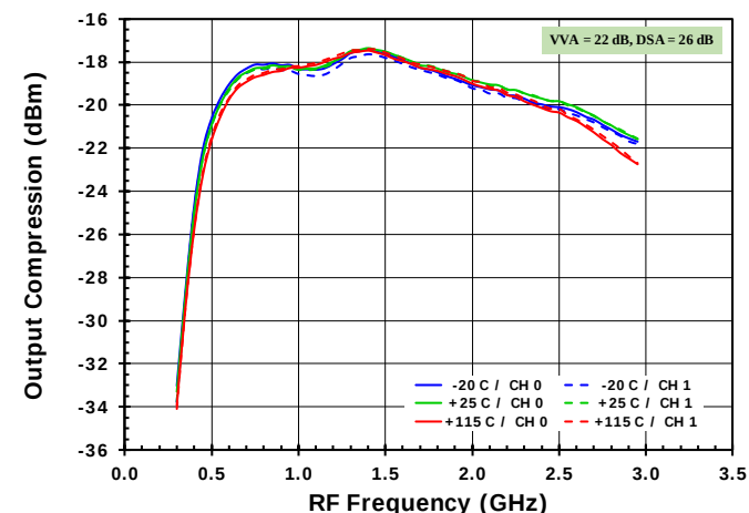
Figure 67. Output P1dB vs Frequency (+3.3V)
