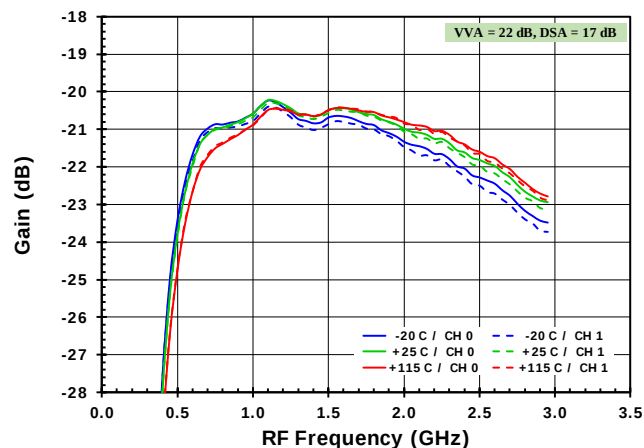
Figure 31. Gain versus Frequency (+3.3V)
