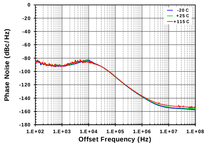
Figure 90. LO Output Phase Noise (2.6550GHz)
