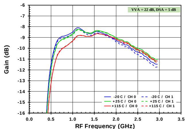
Figure 29. Gain versus Frequency (+3.3V)
