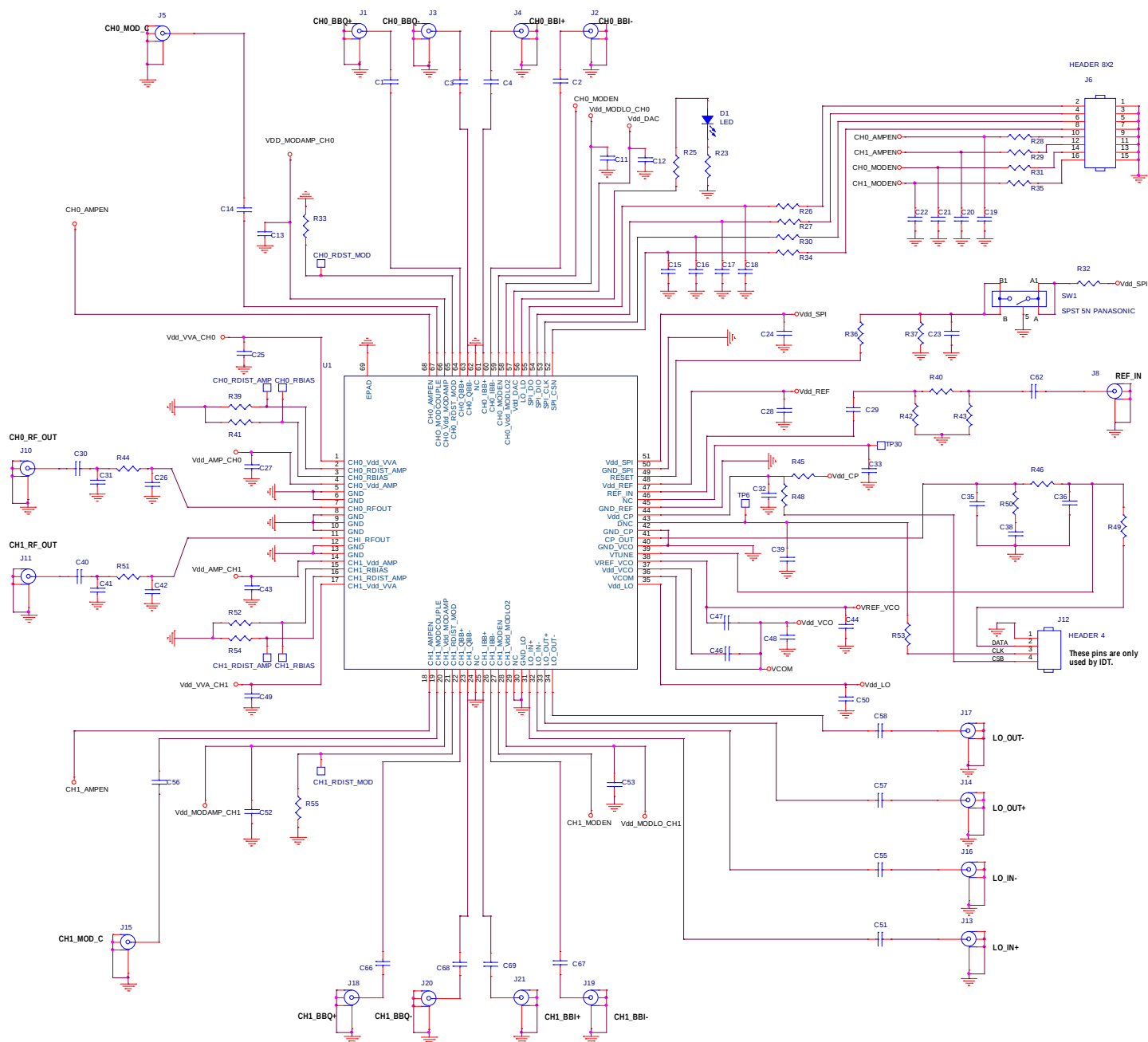
Figure 99. Electrical Schematic for the Differential Evaluation Board
