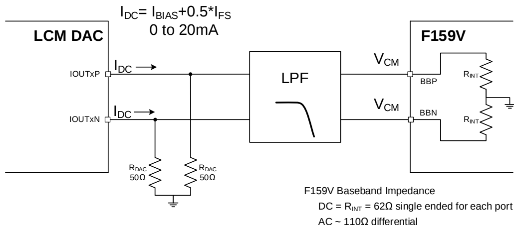
Figure 94. Generic DAC Interface
