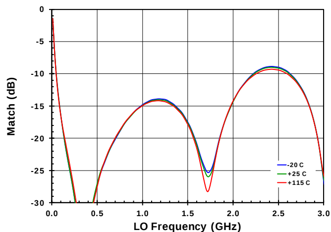
Figure 6. LO Differential Output Return Loss
