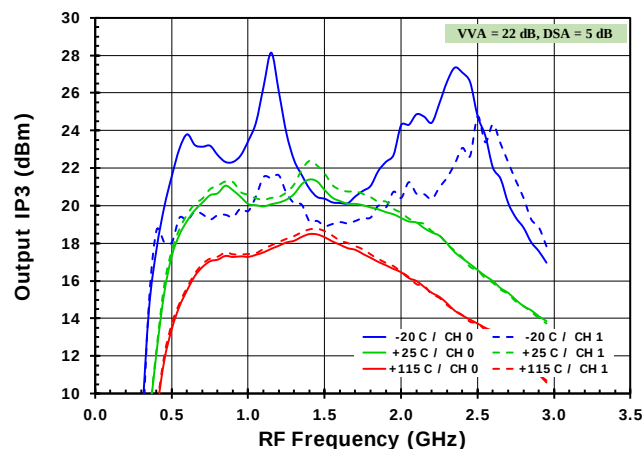
Figure 41. OIP3 versus Frequency (+3.3V)
