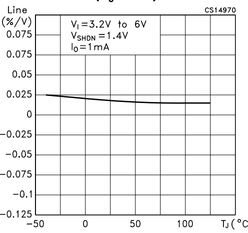
Figure 10. Line regulation vs. temperature ( V_0=2.7\text{ V} )
