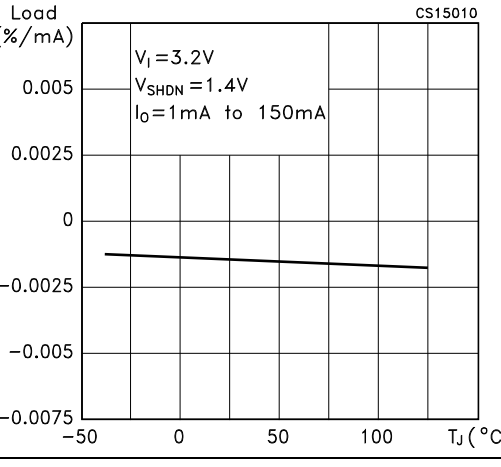
Figure 13. Load regulation vs. temperature ( V_0=2.7\text{ V} )
