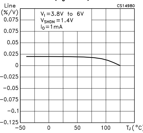
Figure 11. Line regulation vs. temperature ( V_0=3.3\text{ V} )
