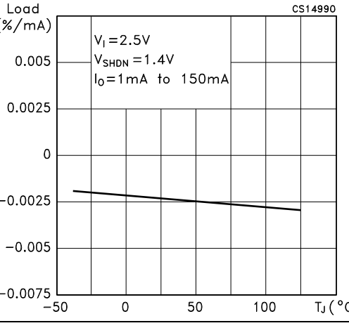
Figure 12. Load regulation vs. temperature ( V_0=1.35\text{ V} )
