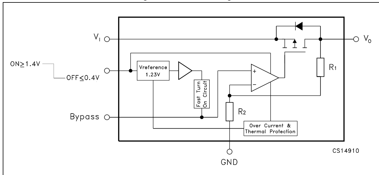
Figure 1. Schematic diagram
