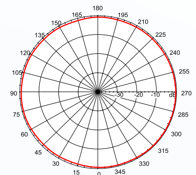
H PLANE 2.45 GHz
