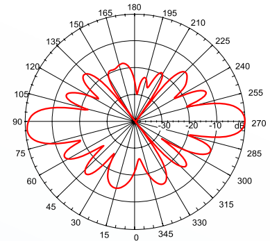
E- PLANE 2.45 GHz
