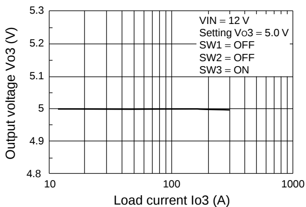
Output Voltage vs. Load Current (CH3)
