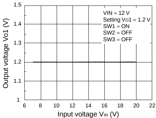
Output Voltage vs. Input Voltage (CH1)
