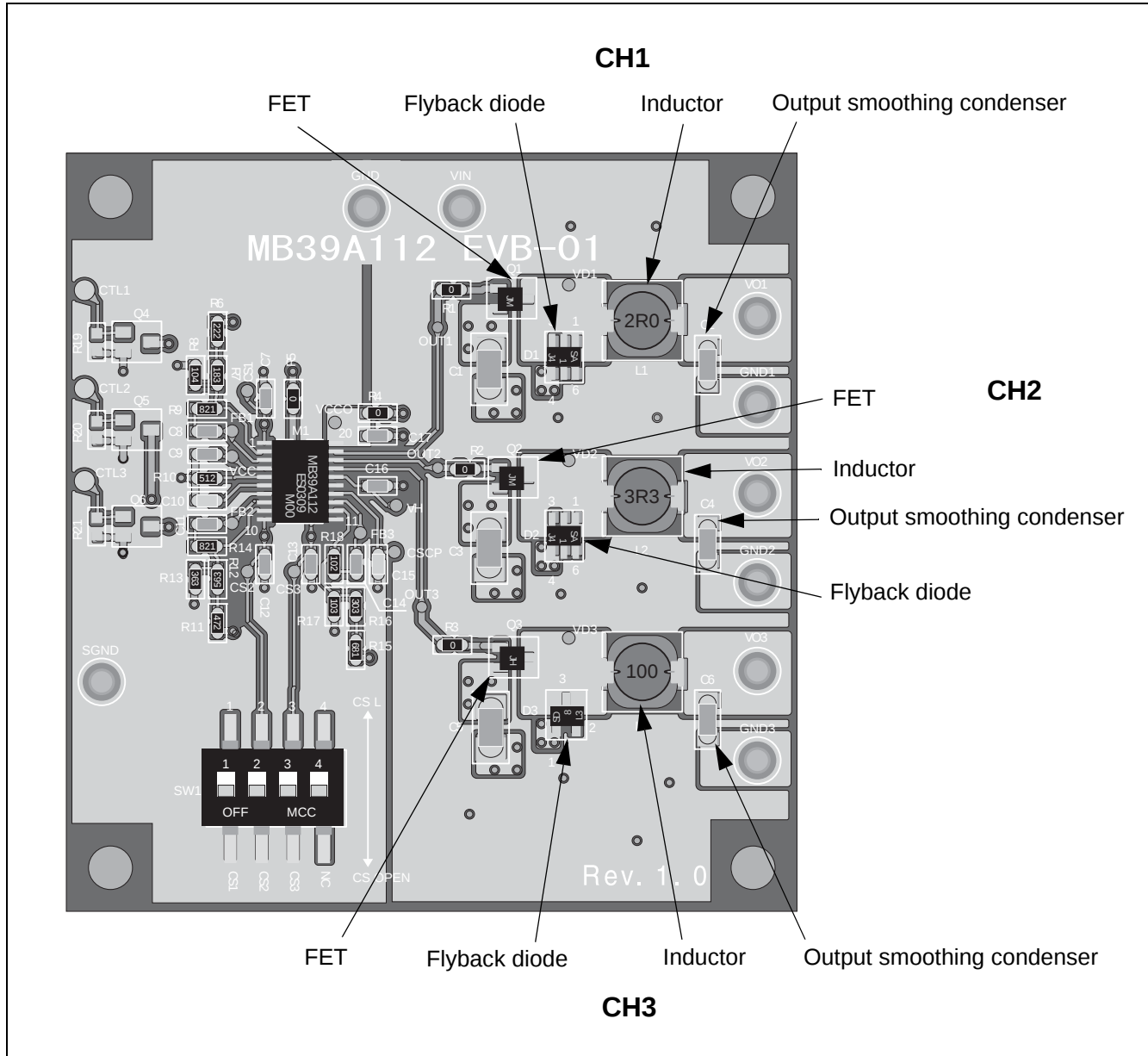
Figure 1. Board Photograph
