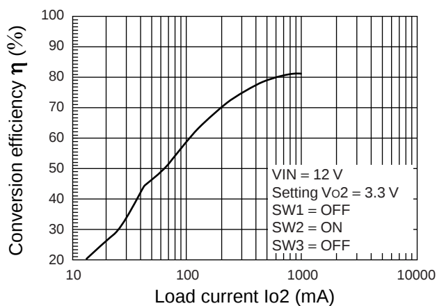
Conversion Efficiency vs. Load Current (CH2)
