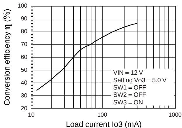
Conversion Efficiency vs. Load Current (CH3)
