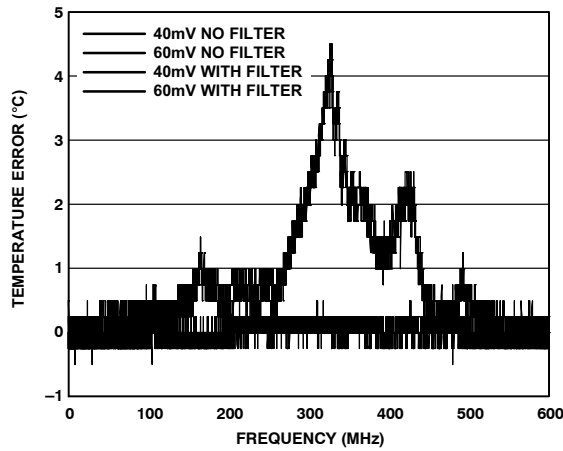
Figure 9. Temperature Error vs. Common-Mode Noise Frequency (With and Without R-C-R Filter of 100 \Omega –2.2 nF–100 \Omega )
