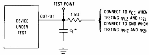
Figure 4. Test Circuit
