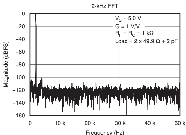
Figure 86. 2-kHz FFT
