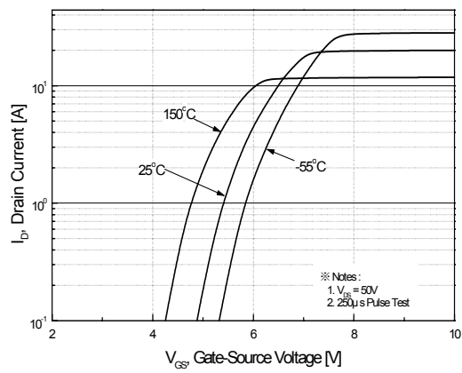
Fig. 2. Transfer characteristics
