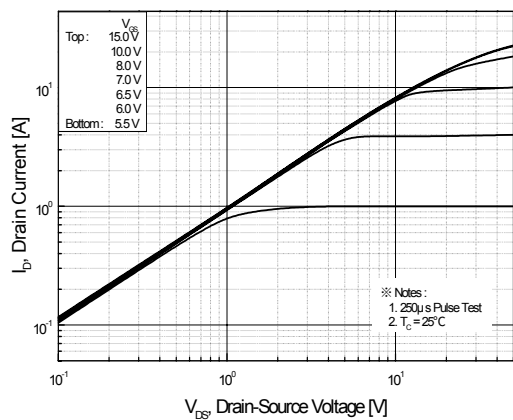
Fig. 1. On-state characteristics
