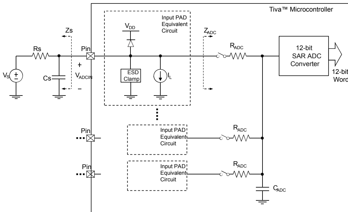
Figure 28-29. ADC Input Equivalency
