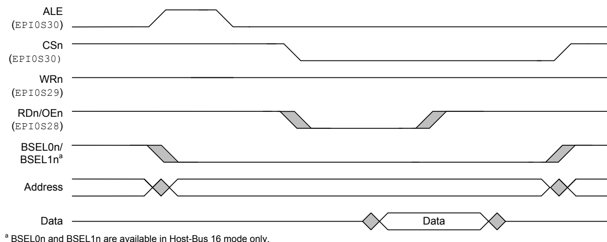
Figure 11-12. Host-Bus Read Cycle, MODE = 0x1, WRHIGH = 0, RDHIGH = 0
