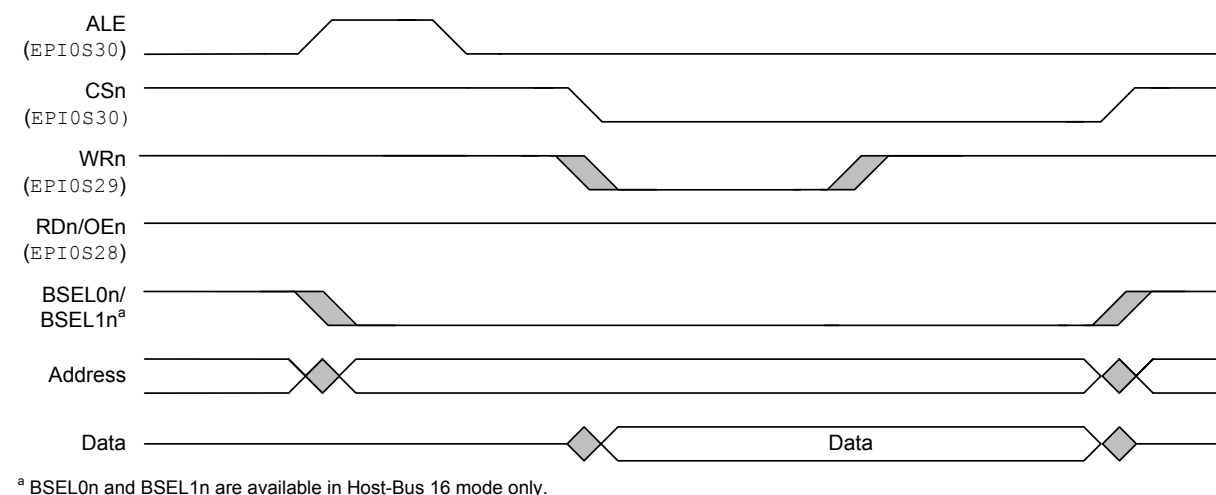
Figure 11-13. Host-Bus Write Cycle, MODE = 0x1, WRHIGH = 0, RDHIGH = 0
