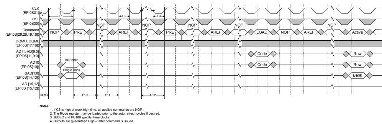
Figure 28-18. SDRAM Initialization and Load Mode Register Timing
