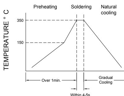
Figure 2. Iron Soldering
