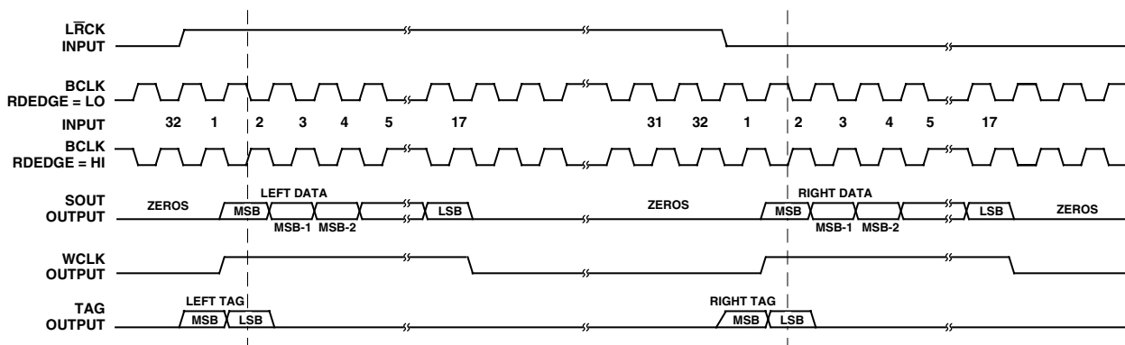
Figure 10. Serial Data Output Timing: Slave Mode, \overline{P}S -Justified, S\overline{M} = HI , RLJUST = LO , MSBDLY = LO
