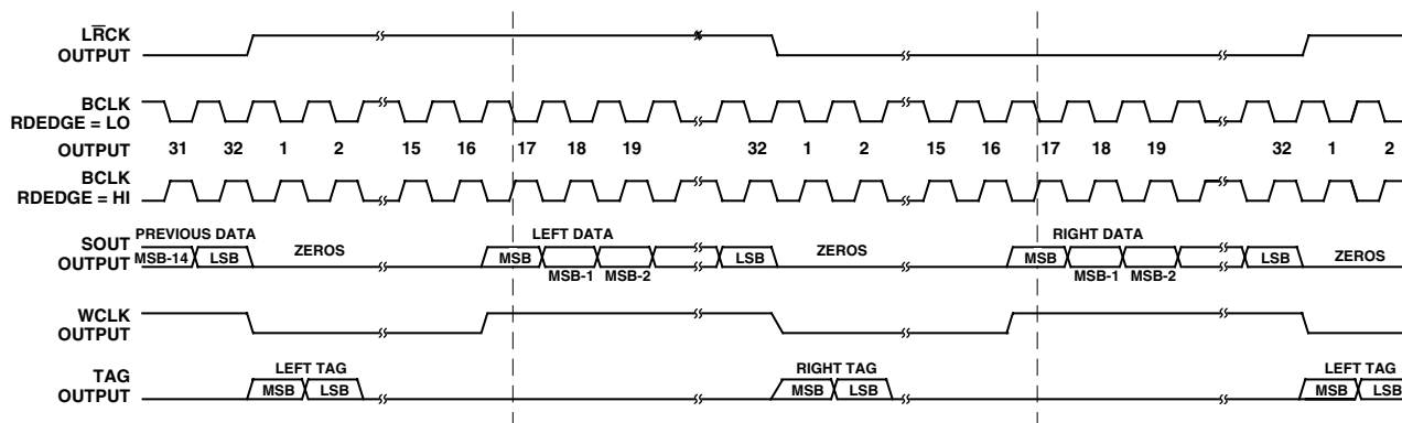
Figure 11. Serial Data Output Timing: Master Mode, Right-Justified with No MSB Delay, S\overline{M} = LO , RLJUST = HI , MSBDLY = HI
