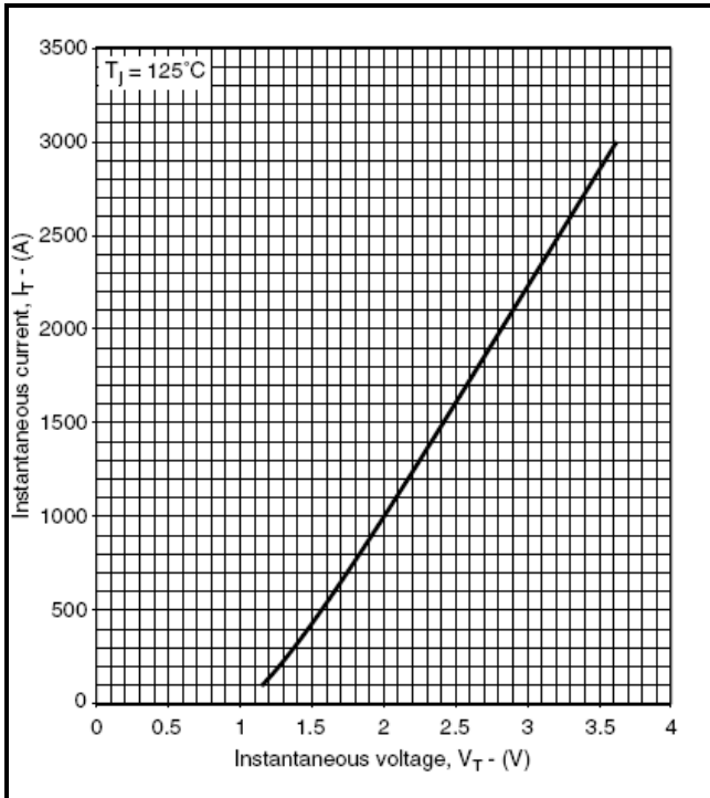
Fig.3 On-state Characteristics
