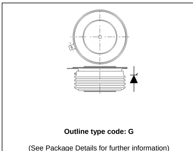
Fig. 1 Package outline
