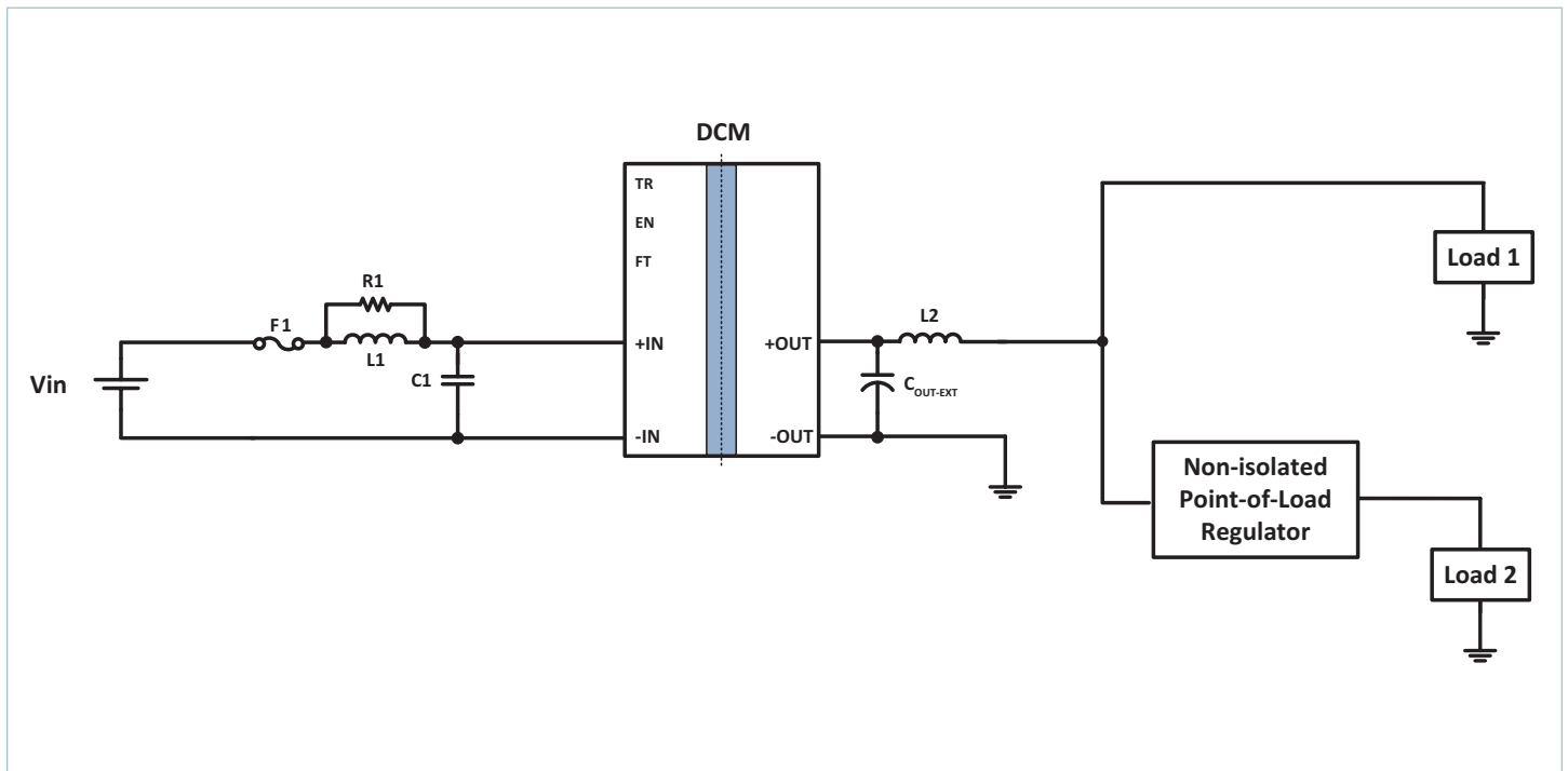
Typical Application: Single DCM4623xD2K06B5y7z, to a non-isolated regulator, and direct to load
