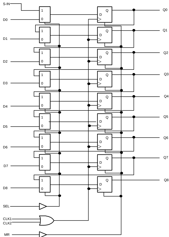
LOGIC SYMBOL
