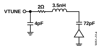
Figure 6. VTUNE Interface
