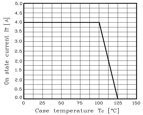
Fig. 2 I_{T(RMS)} - T_C
