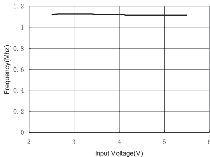
8. Frequency VS Input Voltage
