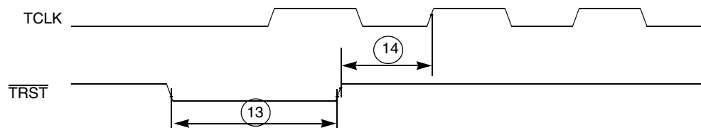
Figure 15. TRST Timing
