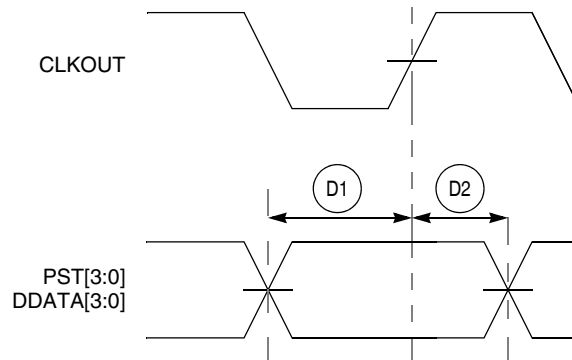
Figure 16. Real-Time Trace AC Timing
