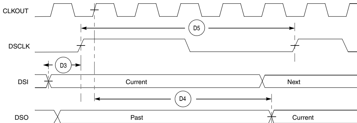
Figure 17. BDM Serial Port AC Timing
