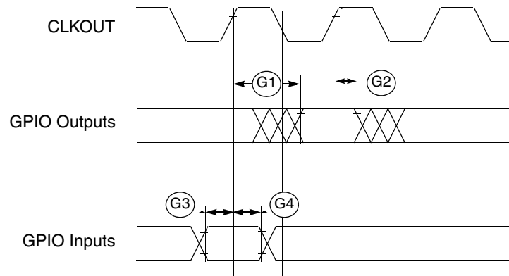
Figure 6. GPIO Timing
