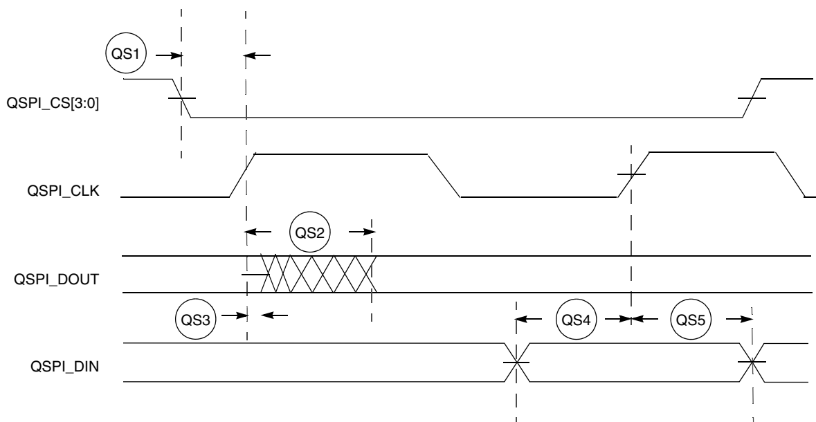
Figure 11. QSPI Timing
