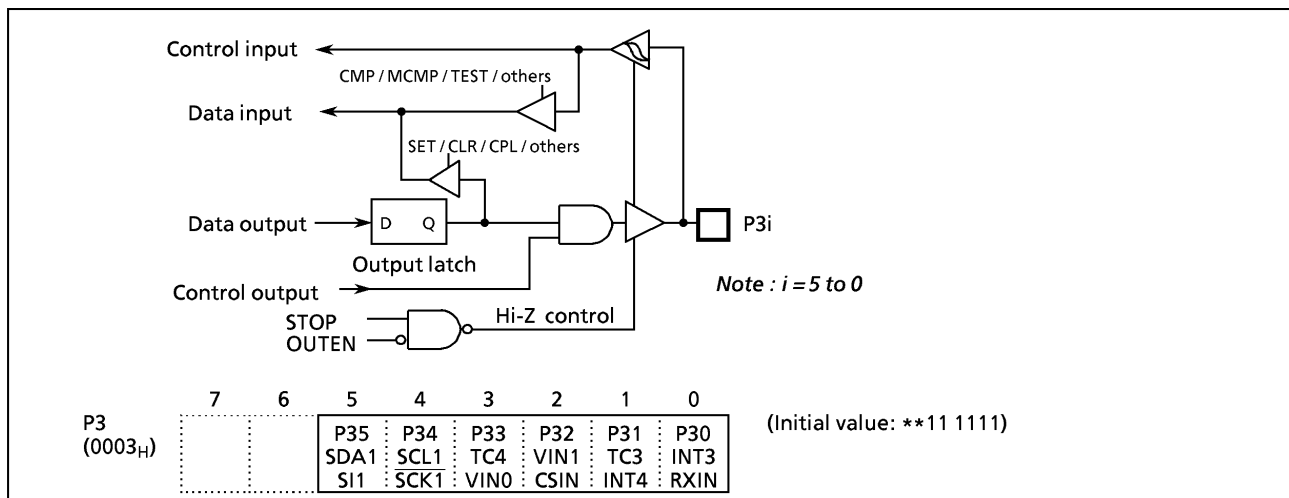
Figure 2-4. Port P3
