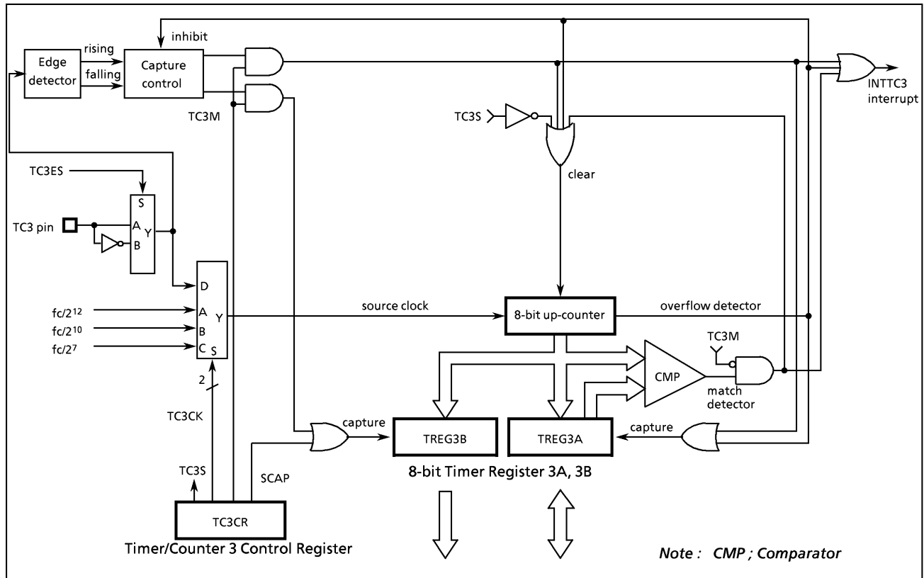
Figure 2-21. Timer/Counter (TC3)
