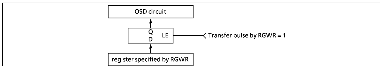
Figure 2-82. RGWR System
