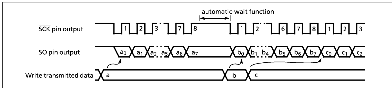
Figure 2-42. Automatic-wait Function
