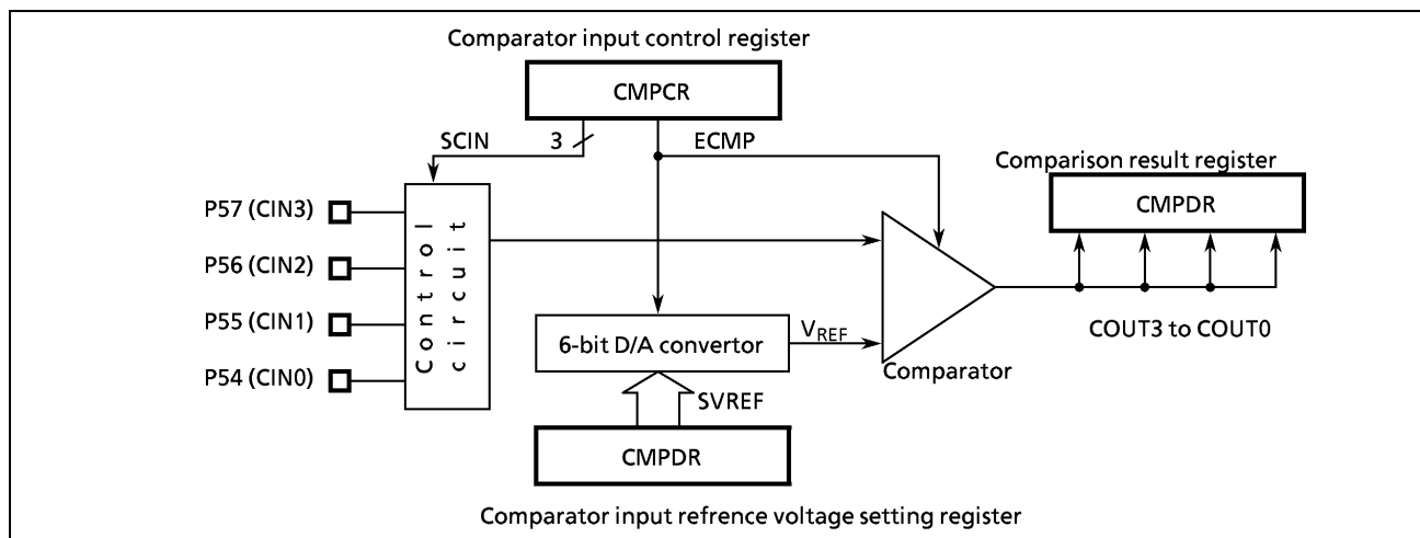
Figure 2-58. 6-bit A/D Conversion (Comparator) Input
