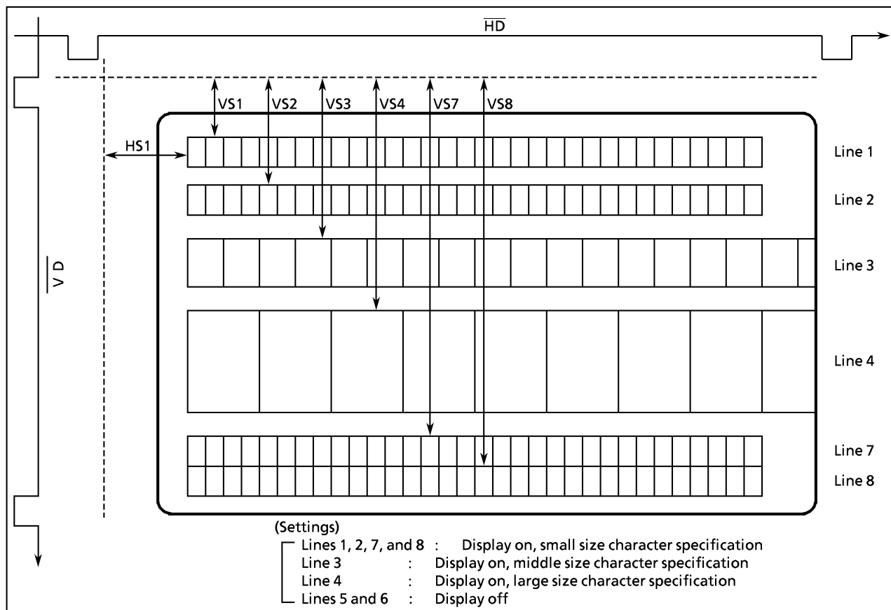
Figure 2-69. TV Screen Display Image
