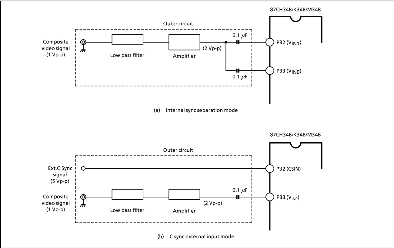
Figure 2-88. Video Signal Connection
