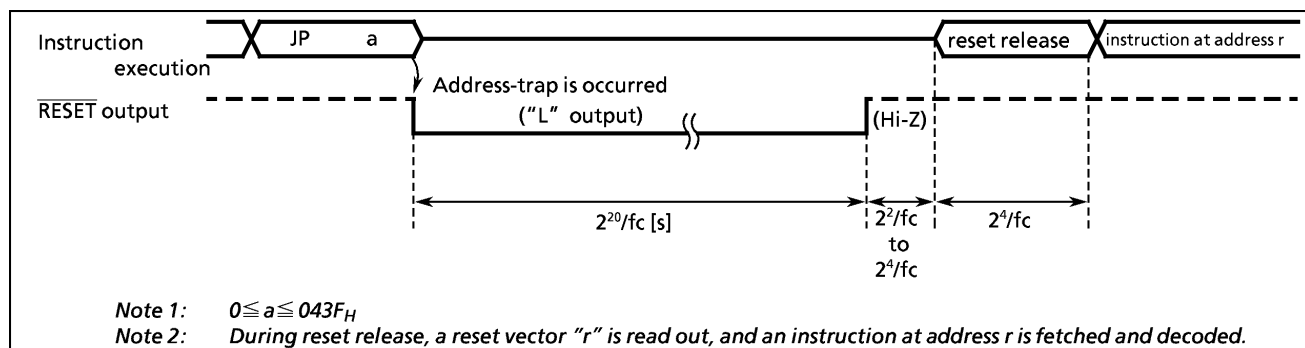
Figure 1-29. Address-Trap-Reset
