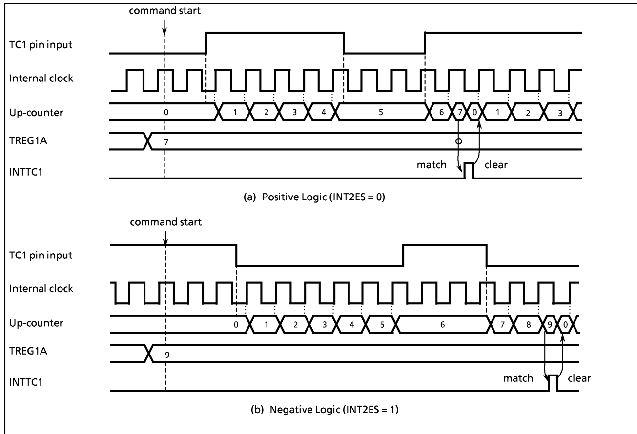
Figure 2-16. Window Mode Timing Chart
