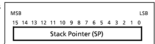
Figure 1-7. Stack Pointer
