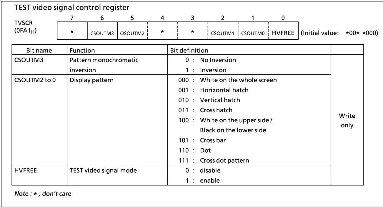
Figure 2-93. TEST Video Signal Control Register
