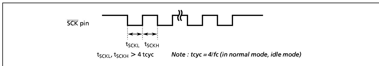
Figure 2-43. External Clock
