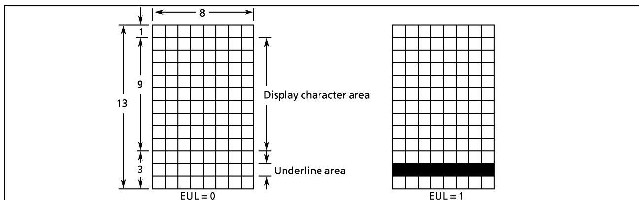
Figure 2-77. Underline
