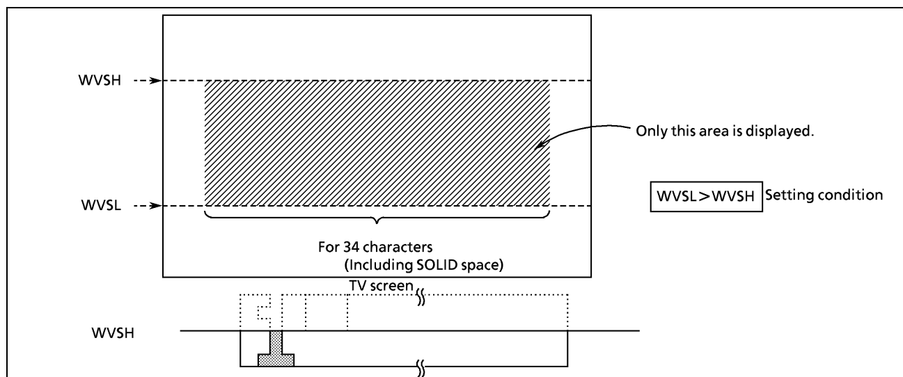
Figure 2-80. Window
