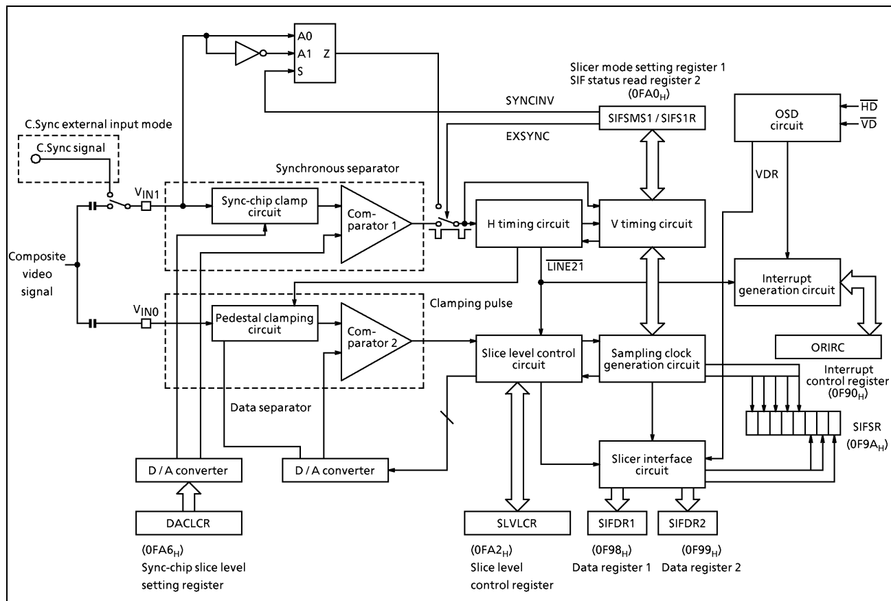
Figure 2-86. Data Slicer
