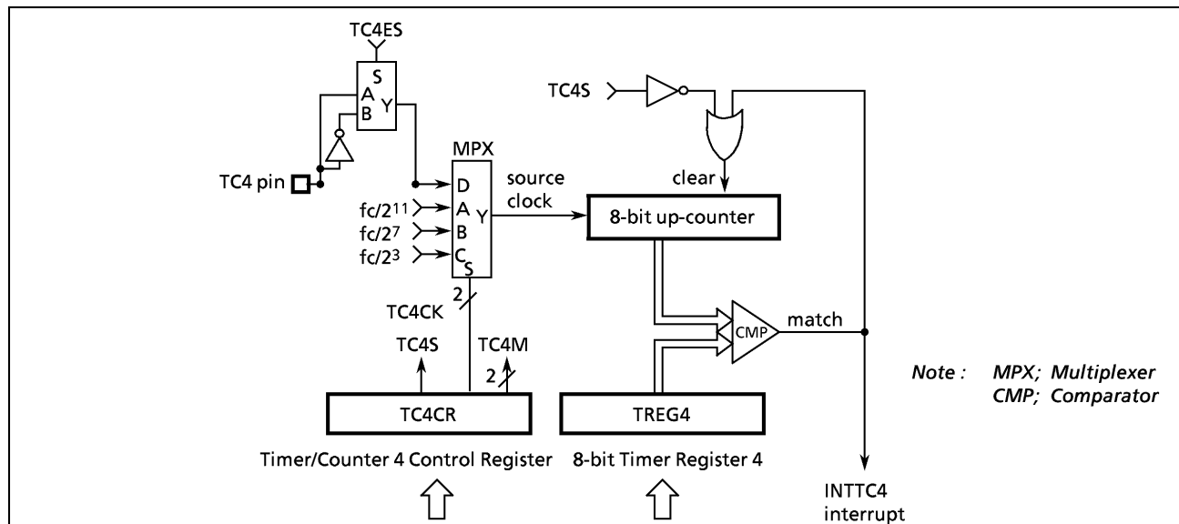
Figure 2-24. Timer/Counter 4
