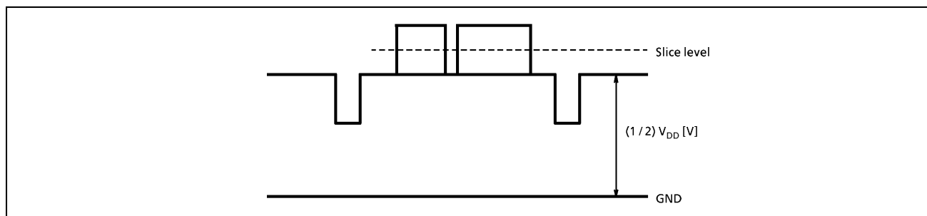
Figure 2-91. Pedestal Clamp
