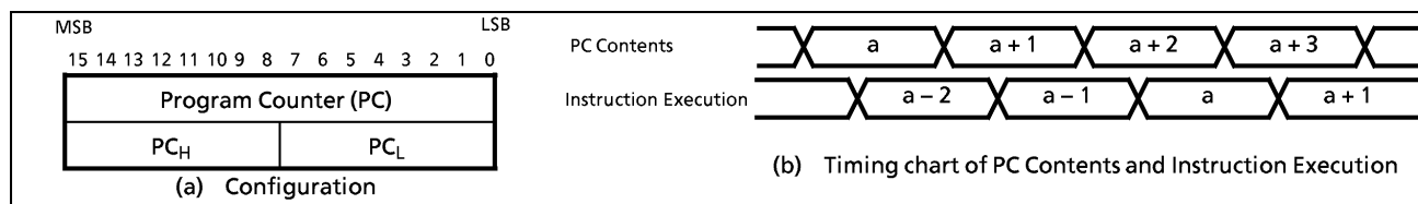
Figure 1-3. Program Counter
