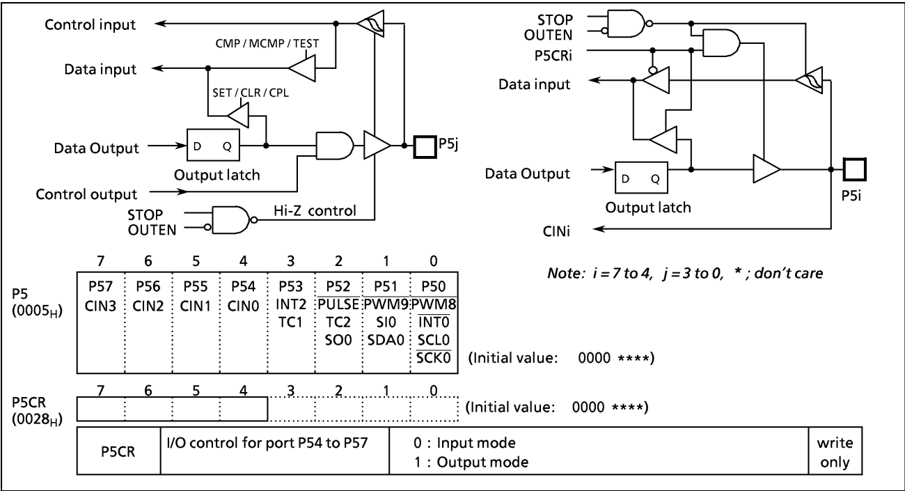
Figure 2-6. Ports P5
