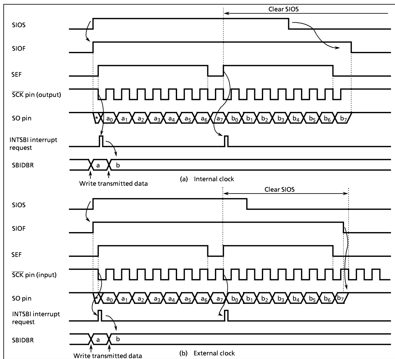
Figure 2-45. Transfer Mode
