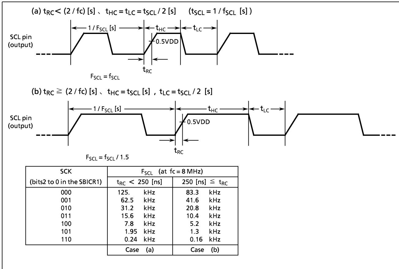
Figure 2-32. Serial Clock
