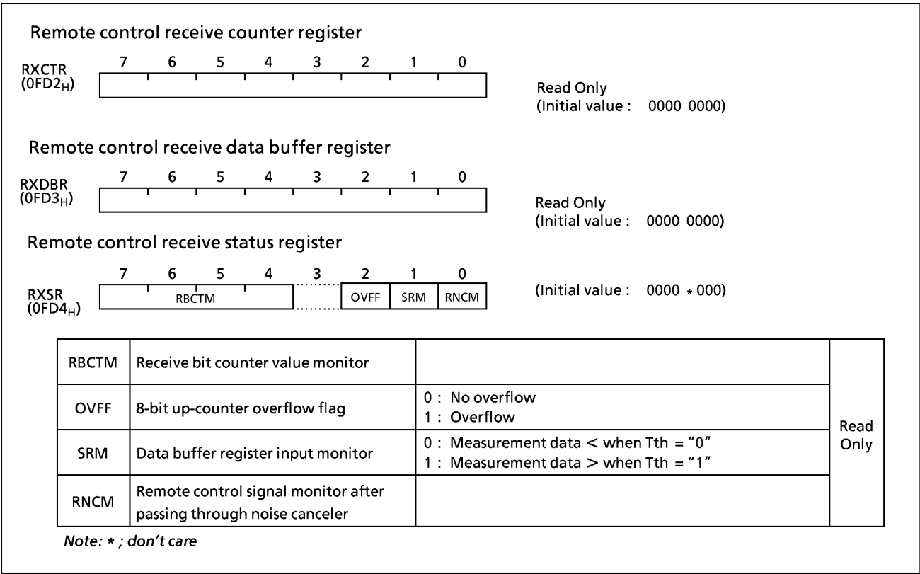
Figure 2-52. Remote Control Receive Counter Register, Data Buffer Register, Status Register
