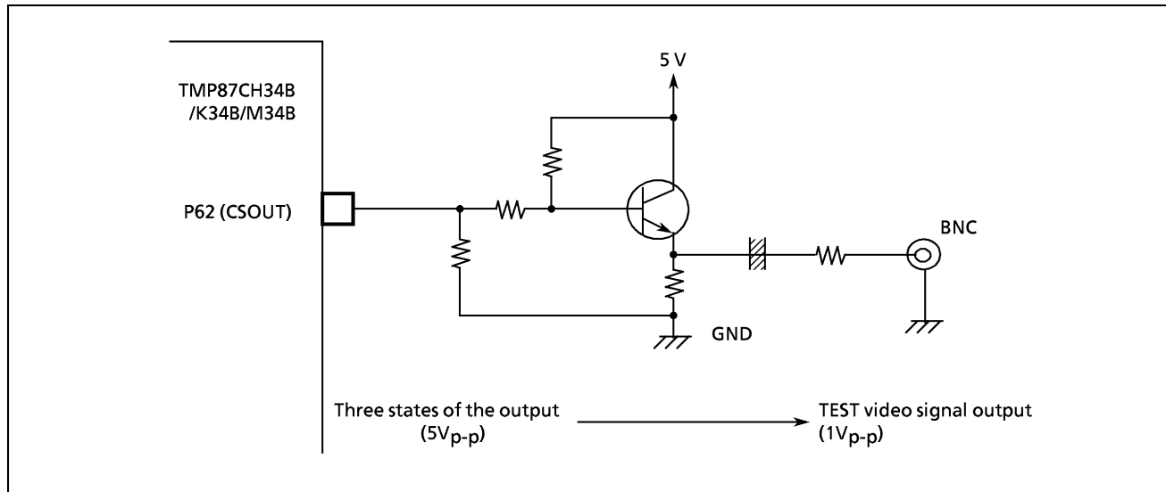
Figure 2-95. Example of Test Video Output Generation
