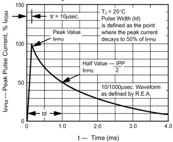
Fig. 3 – Pulse Waveform
