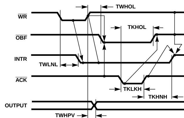
FIGURE 18. MODE 1 (STROBED OUTPUT)
