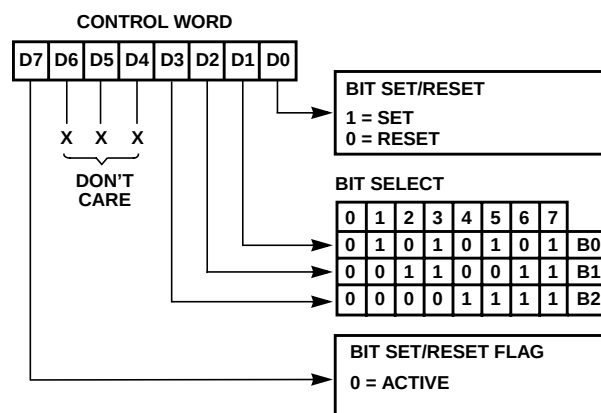
FIGURE 12. BIT SET/RESET CONTROL WORD FORMAT
