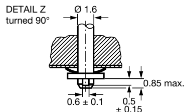
Trimmers BFC2 809 090.. series, with one rotor contact
