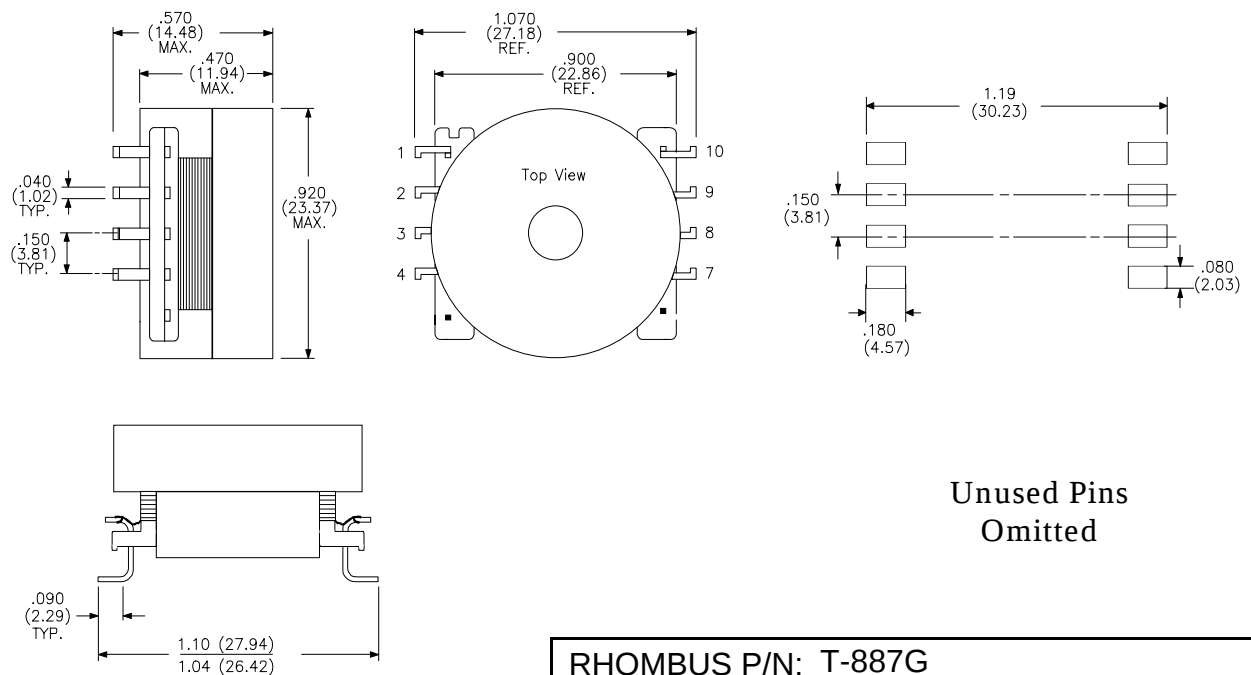
Physical Dimensions inches (mm)
