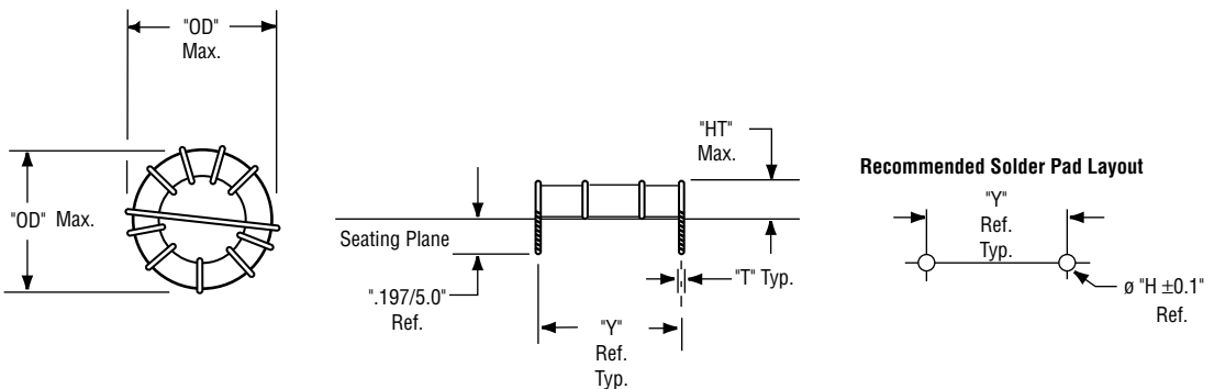
Figure 2 - Horizontal Mount
