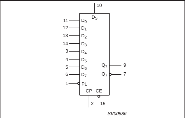
LOGIC SYMBOL
