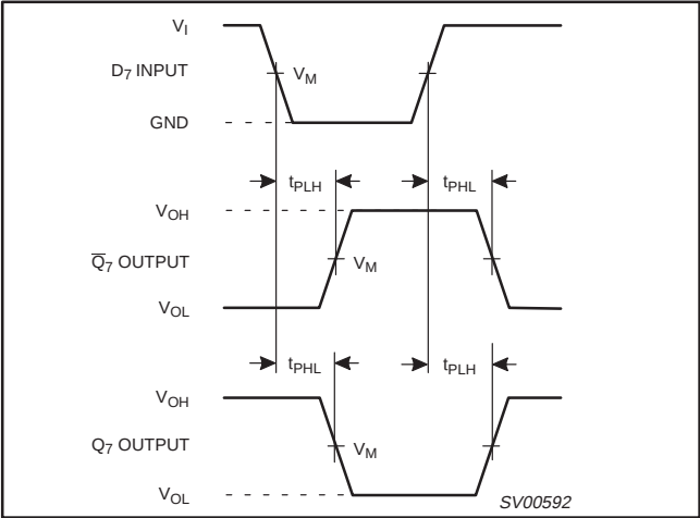
Figure 3. Data input ( D_n ) to output ( Q_7 or \overline{Q}_7 ) propagation delays when \overline{PL} is LOW.
