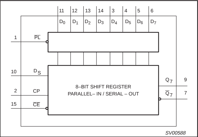
FUNCTIONAL DIAGRAM
