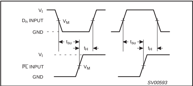
Figure 5. Set-up and hold times from the data inputs ( D_n ) to the parallel load input ( \overline{PL} ).
