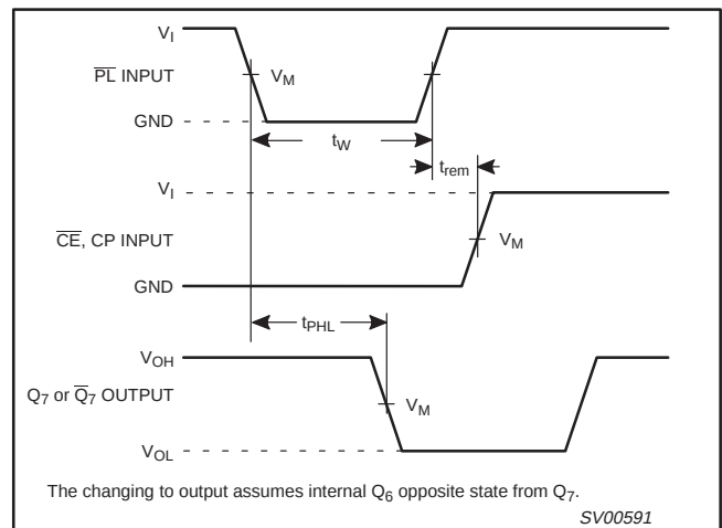
Figure 2. Parallel load ( \overline{PL} ) pulse width, the parallel load to output ( Q_7 or \overline{Q}_7 ) propagation delays, the parallel load to clock (CP) and clock enable (CE) removal time.
