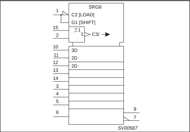
LOGIC SYMBOL (IEEE/IEC)
