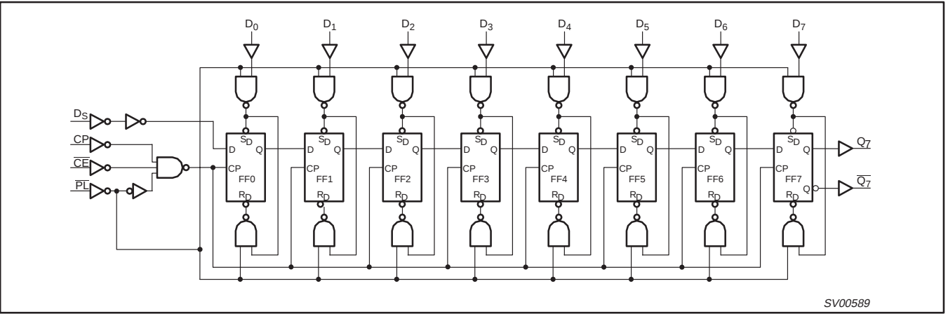
LOGIC DIAGRAM
