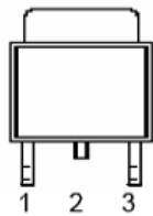
SE5120JTXX 1:GND, 2:OUT, 3:IN
