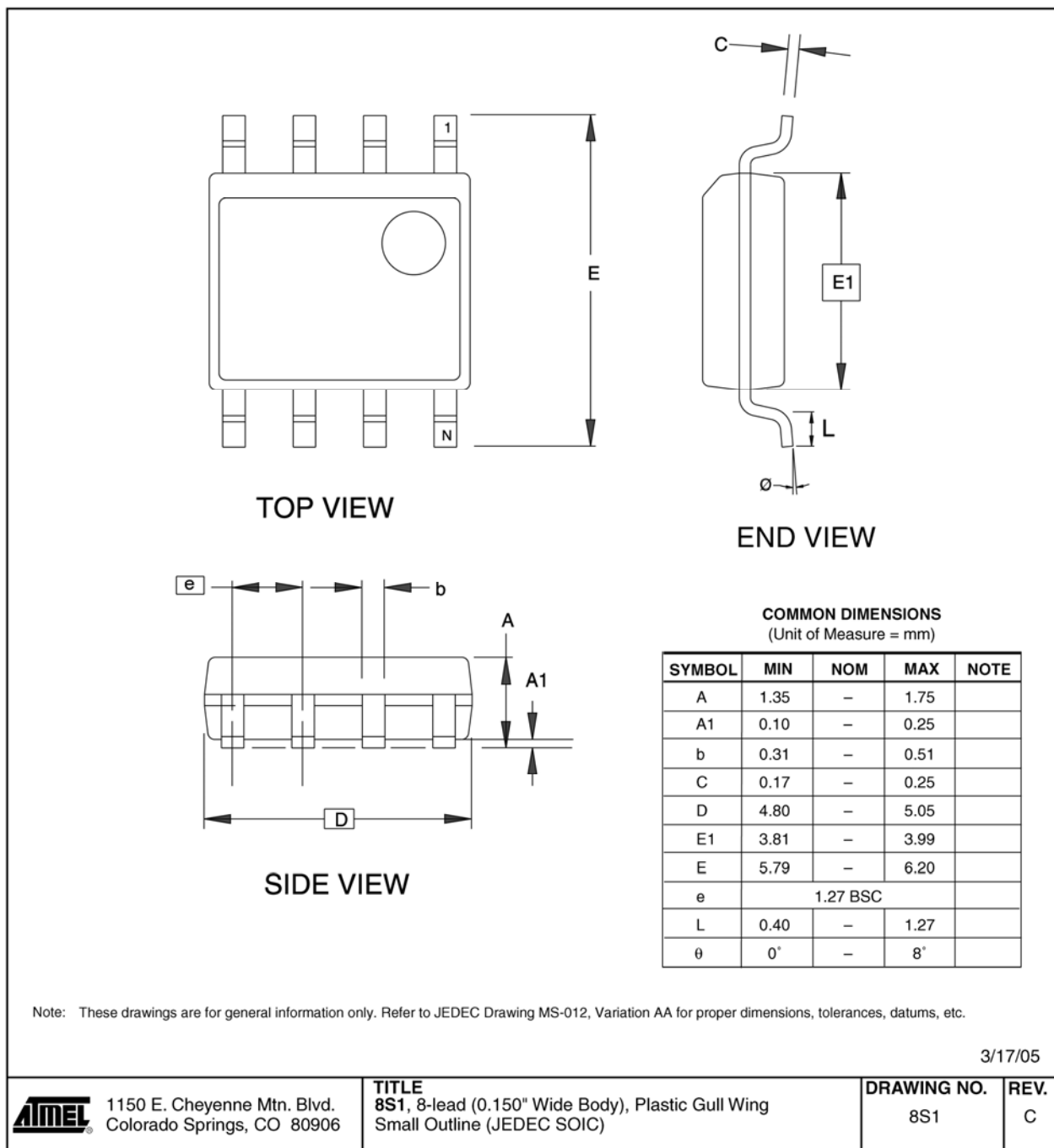
Figure 3. 8S1 – SOIC
