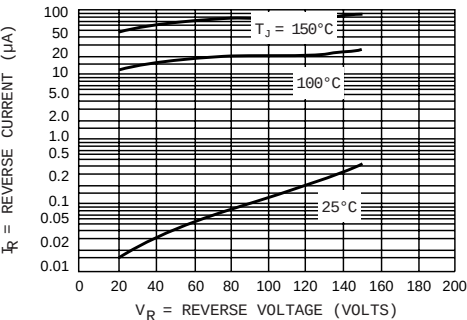
TYPICAL REVERSE CURRENT COM5221, 5222, 5223, 5224
