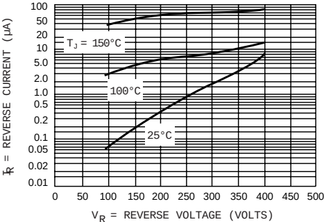
TYPICAL REVERSE CURRENT COM5225, COM5226
