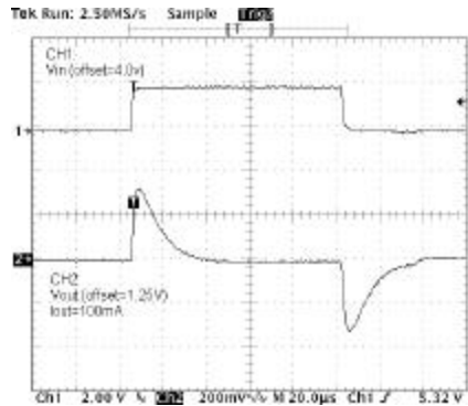
Line transient
