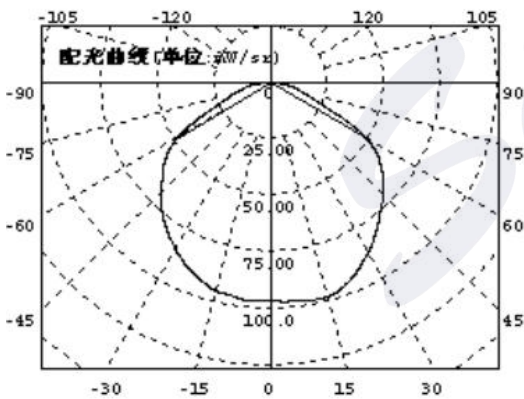
Luminous angle
