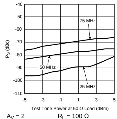
A_V = 2 R_L = 100\ \Omega R_F = 237\ \Omega
