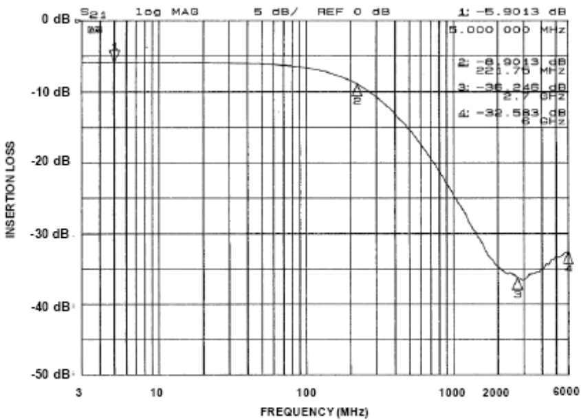
Figure 2. Insertion Loss VS. Frequency (A2-C2 to GND B1)
