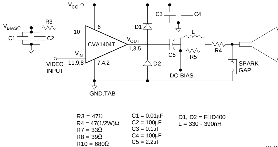
FIGURE 4. APPLICATION CIRCUIT
