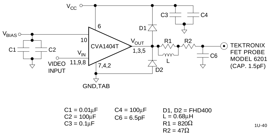
FIGURE 1. TEST CIRCUIT
