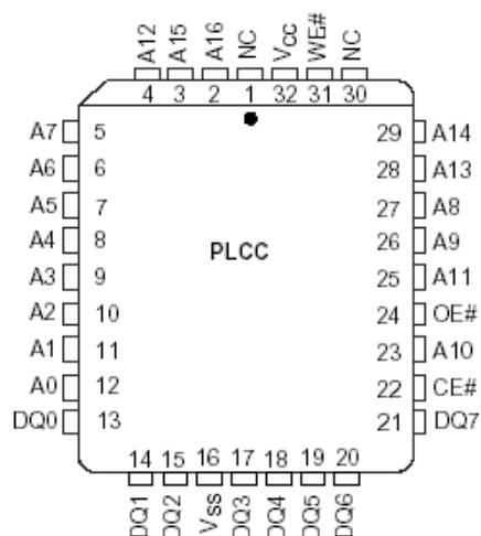
FIGURE 3. PLCC
