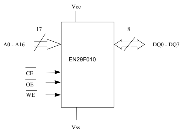
FIGURE 1. LOGIC DIAGRAM
