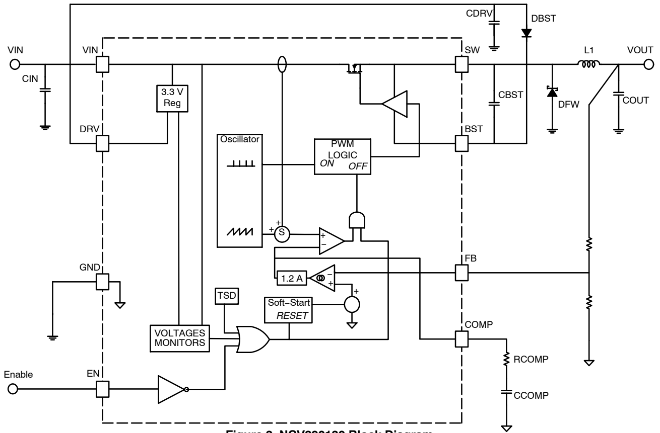
Figure 2. NCV890130 Block Diagram
