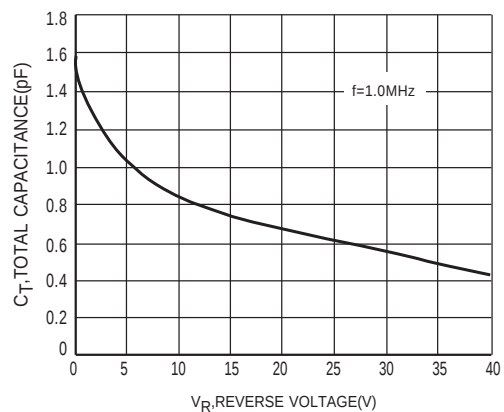
Figure 3 Typical Capacitance
