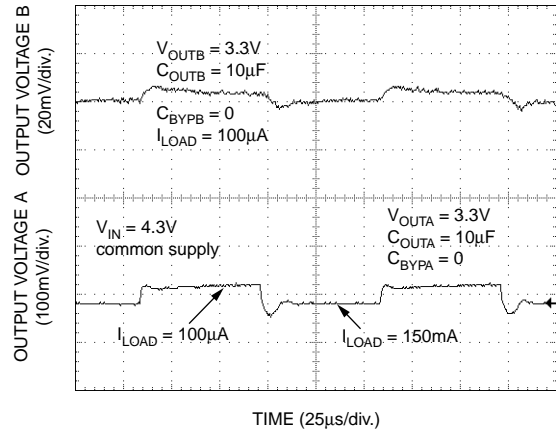
Crosstalk Characteristics
