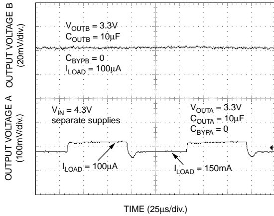
Crosstalk Characteristics
