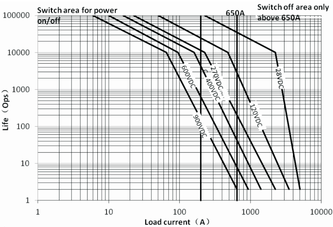
Resistive load life at different voltages
