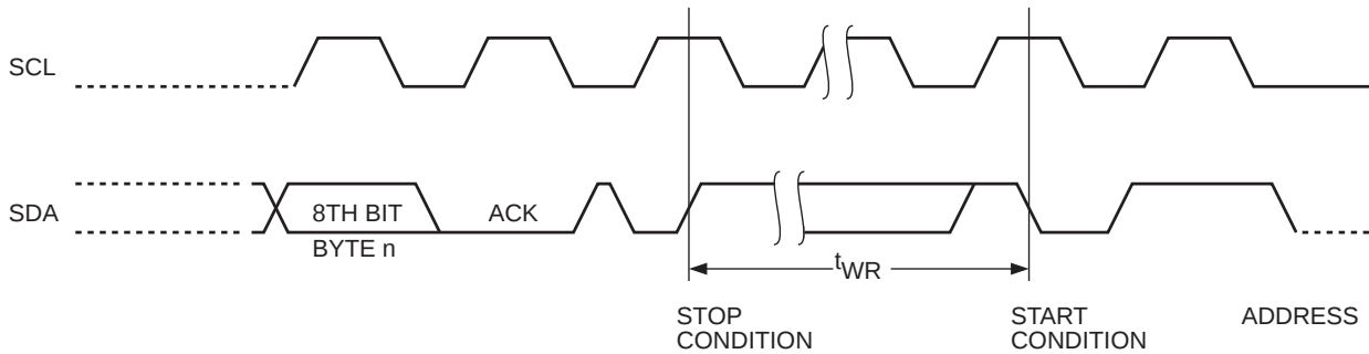
Figure 4. Start/Stop Timing
