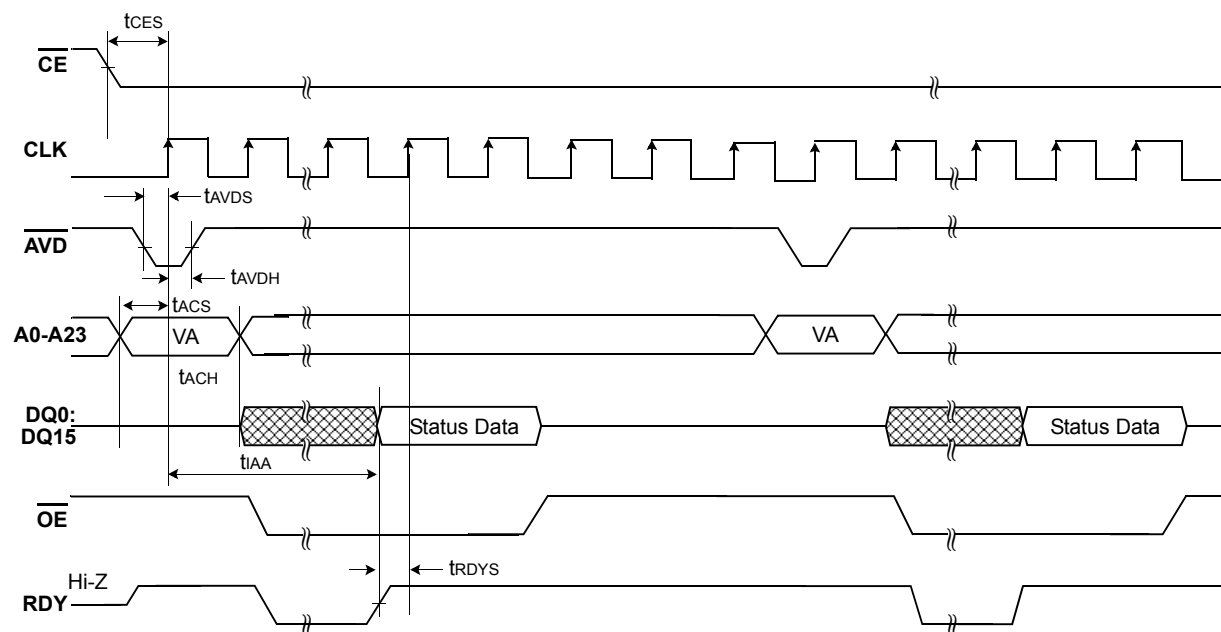
Figure 18: Toggle Bit Timings(During Internal Routine)
