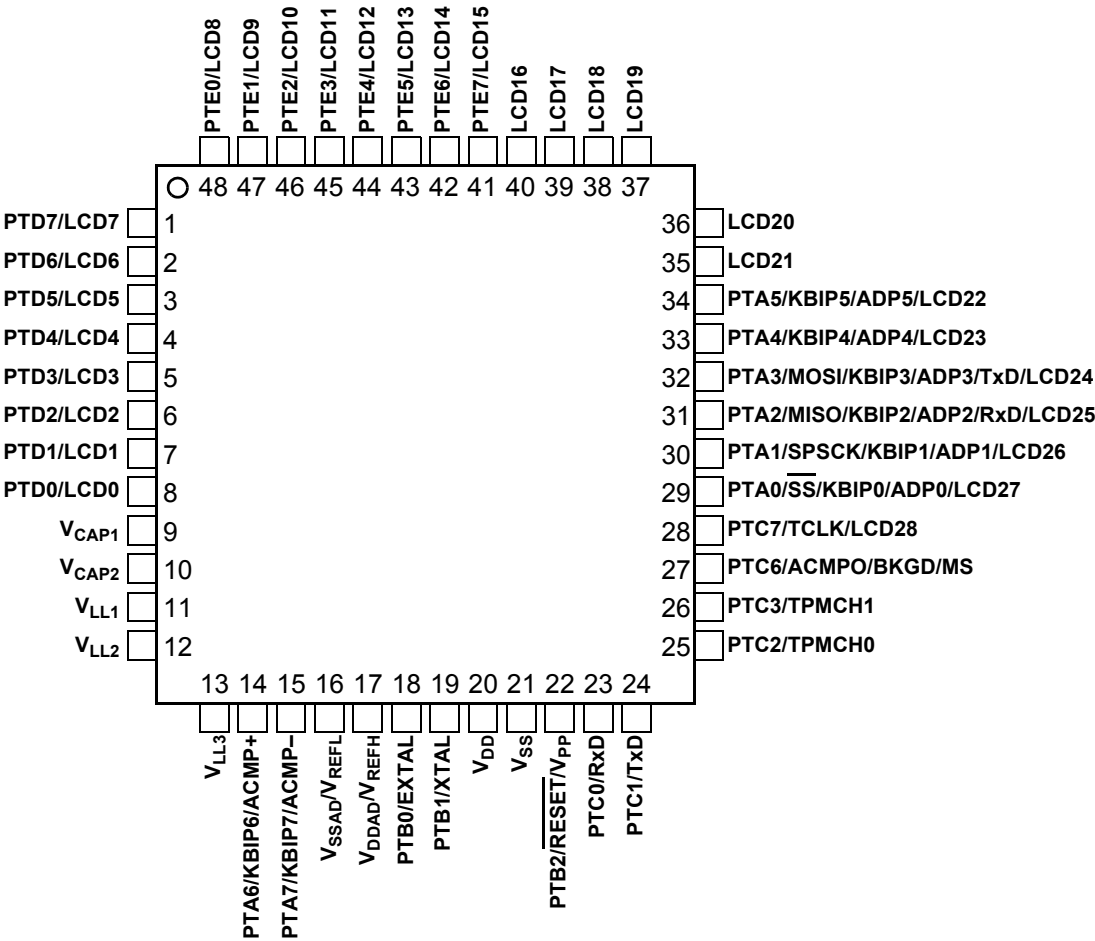
Figure 2. MC9RS08LA8 Series in 48-Pin QFN/LQFP Package
