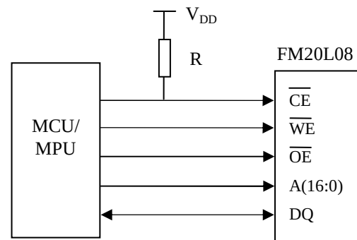
Figure 3. Use of Pullup Resistor on \overline{\text{CE}}
