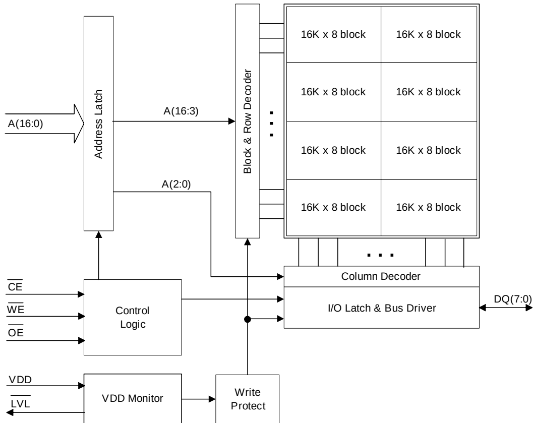
Figure 1. Block Diagram
