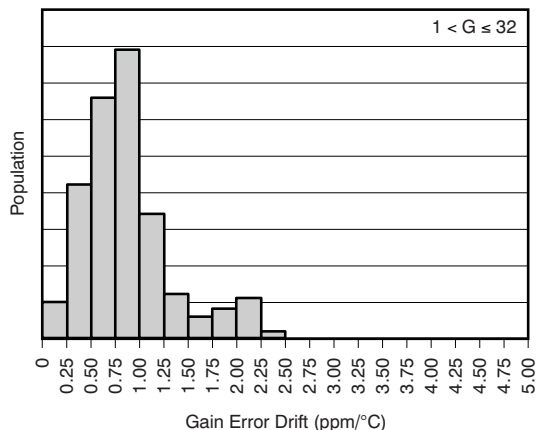
Figure 15. Gain Error Drift ( -40^\circ\text{C} to 125^\circ\text{C} )
