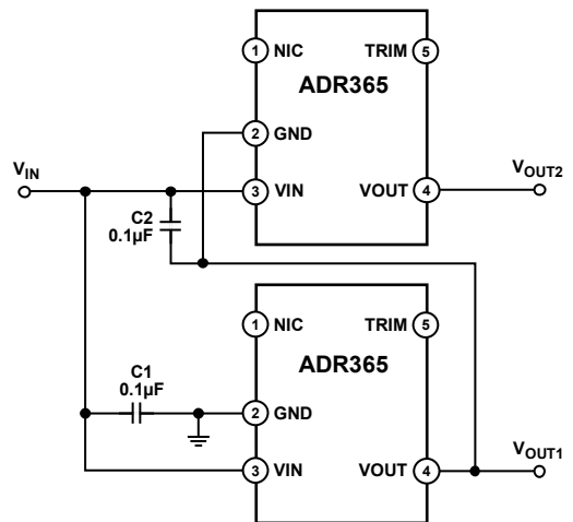
Figure 38. Stacking Voltage References with the ADR365
