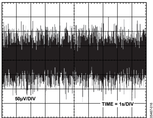
Figure 22. ADR363 10 Hz to 10 kHz Noise
