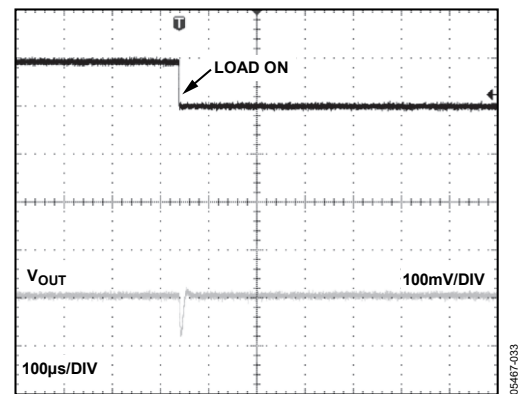
Figure 31. ADR361 Load Transient Response with 0.1 μF Output Capacitor
