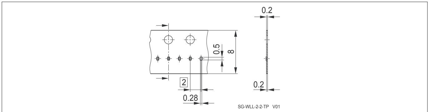
Figure 15 WLL-2-2 packing
