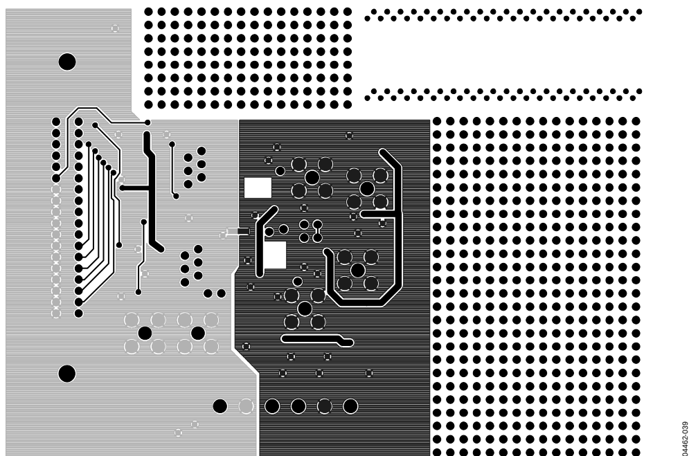
Figure 49. Solder-Side Artwork
