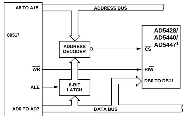
Figure 44. 8xC51-to-AD5428/AD5440/AD5447 Interface
