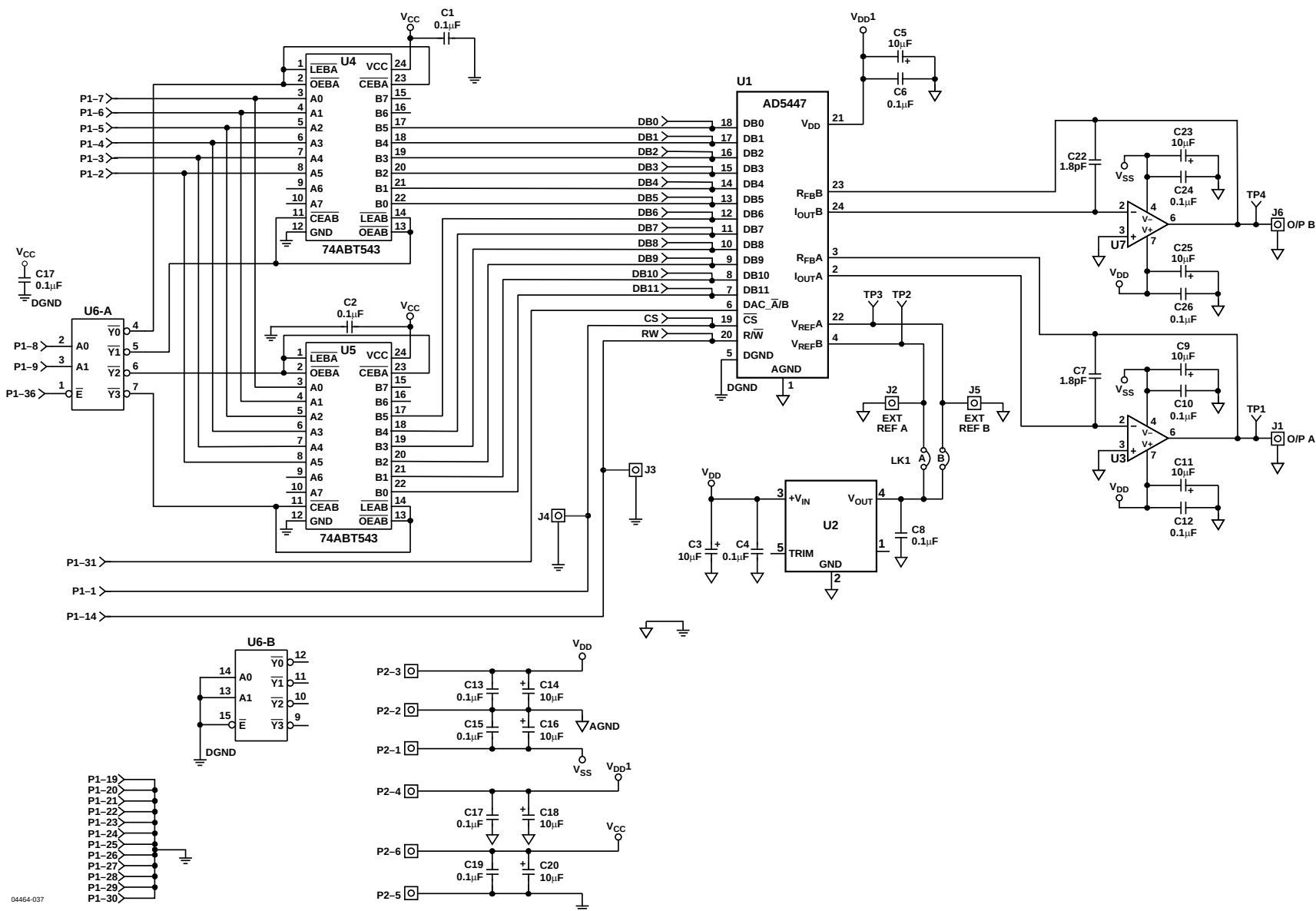
Figure 46. Schematic of AD5447 Evaluation Board
