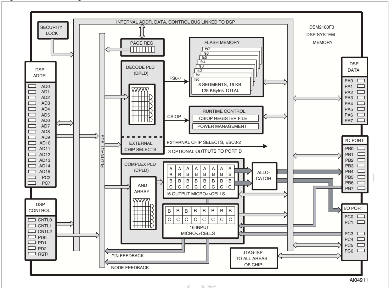
Figure 5. Block Diagram
