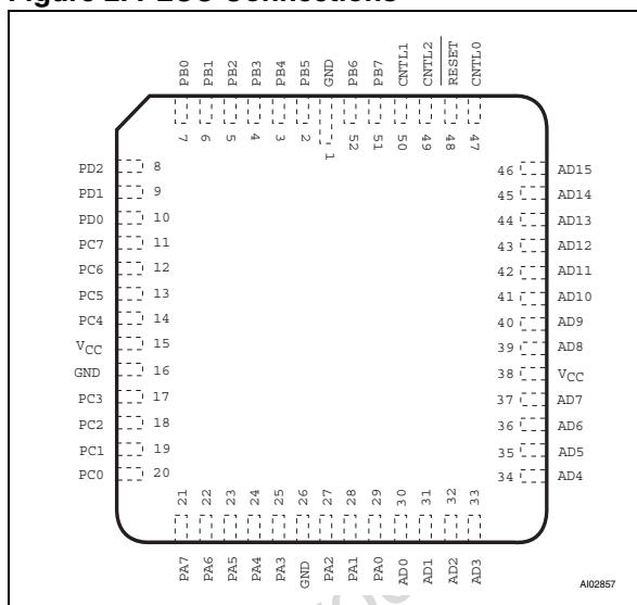
Figure 2. PLC Connections
