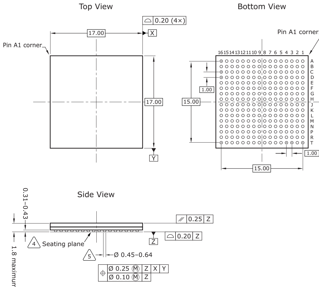
Figure 106 • Package Drawing
